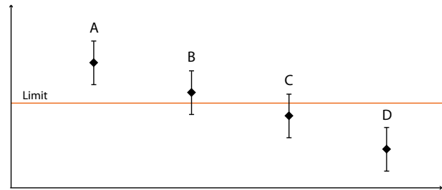
Figure II – Four possible outcomes for conformity assessment decisions
