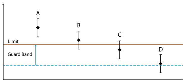
Figure III – Introducing guard band
