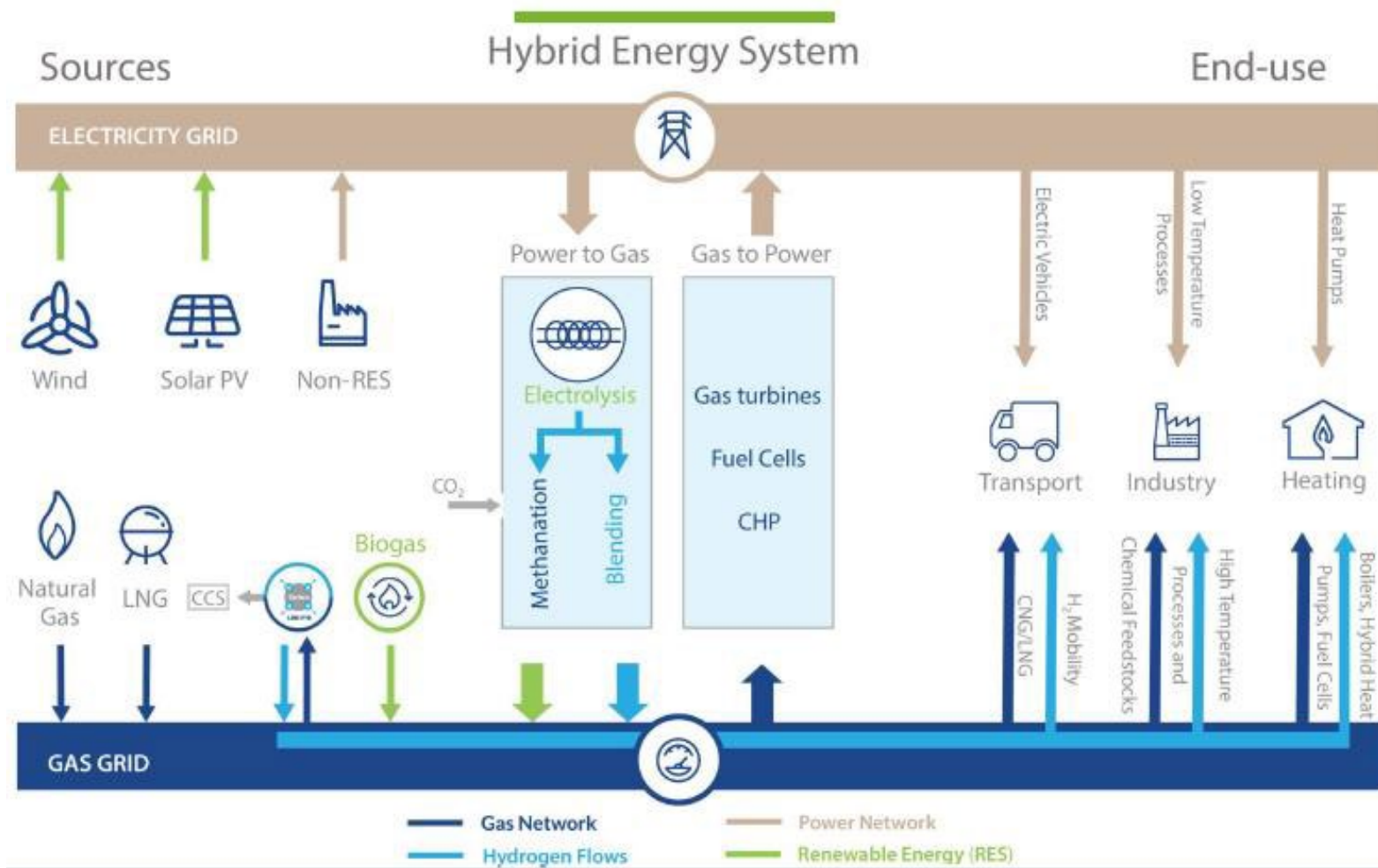
Hybrid Energy System – Enabling VRE through Sectoral Integration/Sector Coupling Source: ENTSOG
