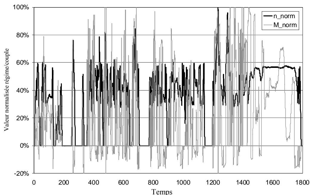
Figure 3. Cycle d'essai WHTC
