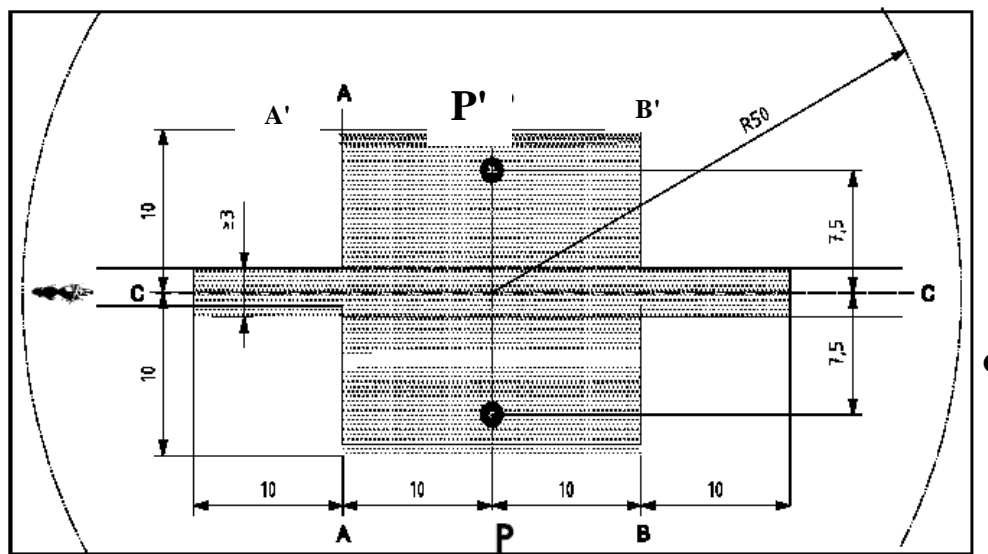
Figure 1 Minimum requirements for test surface area. The shaded part is called "Test Area"
