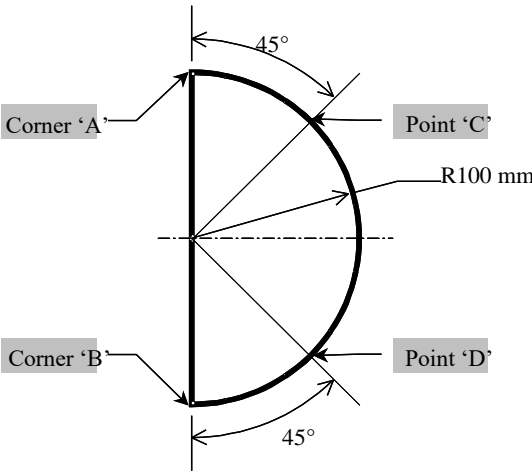
Figure 4 Marking of intersection between bonnet rear and side reference lines
