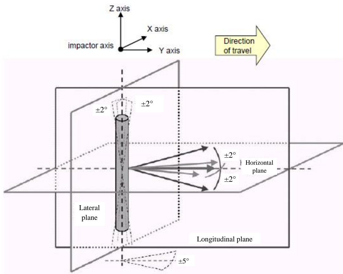
Figure 3 Tolerances of angles for the flexible lower legform impactor at the time of the first impact
