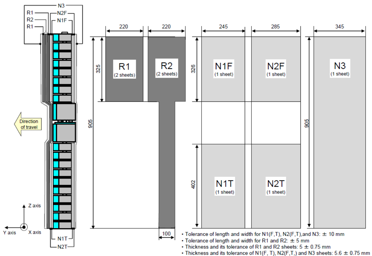
Figure 1 Flexible lower legform impactor: Flesh and skin dimensions
