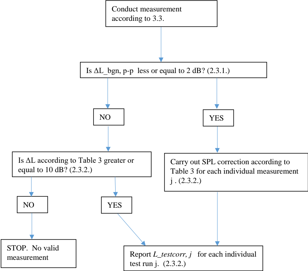
Figure 5 Vehicle A-Weighted sound pressure level measurement correction criteria
