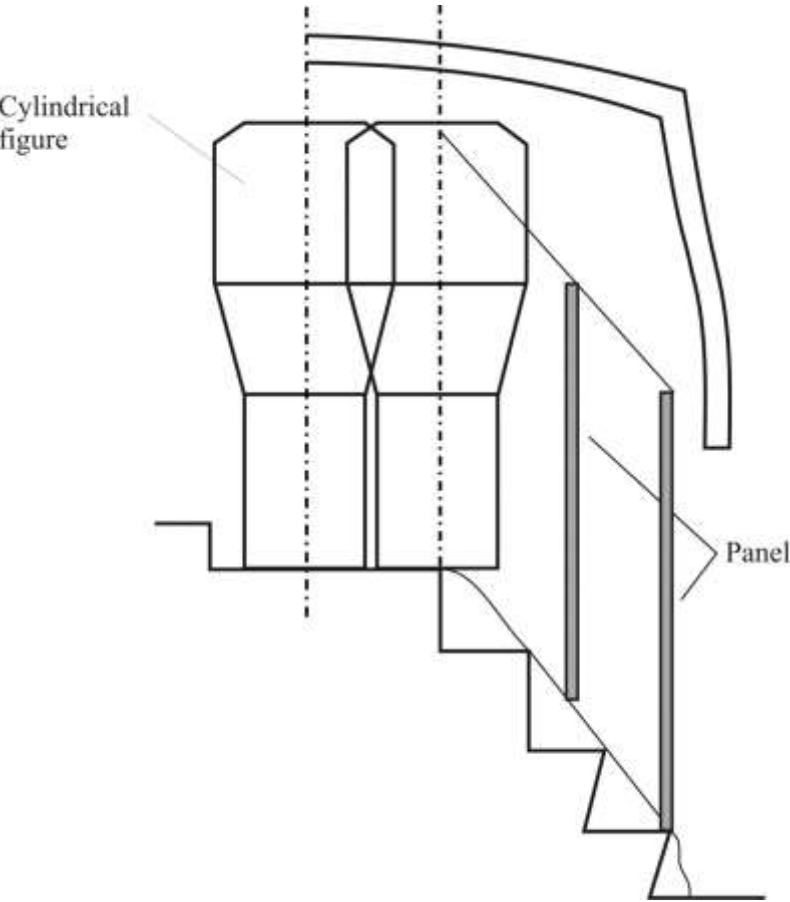
Figure 3 Determination of unobstructed access to door (dimensions in mm) (See Annex 3, paragraph 7.7.1.9.1.)
