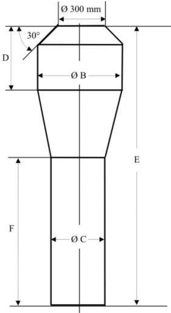
Figure 6 Gangway mannequin
