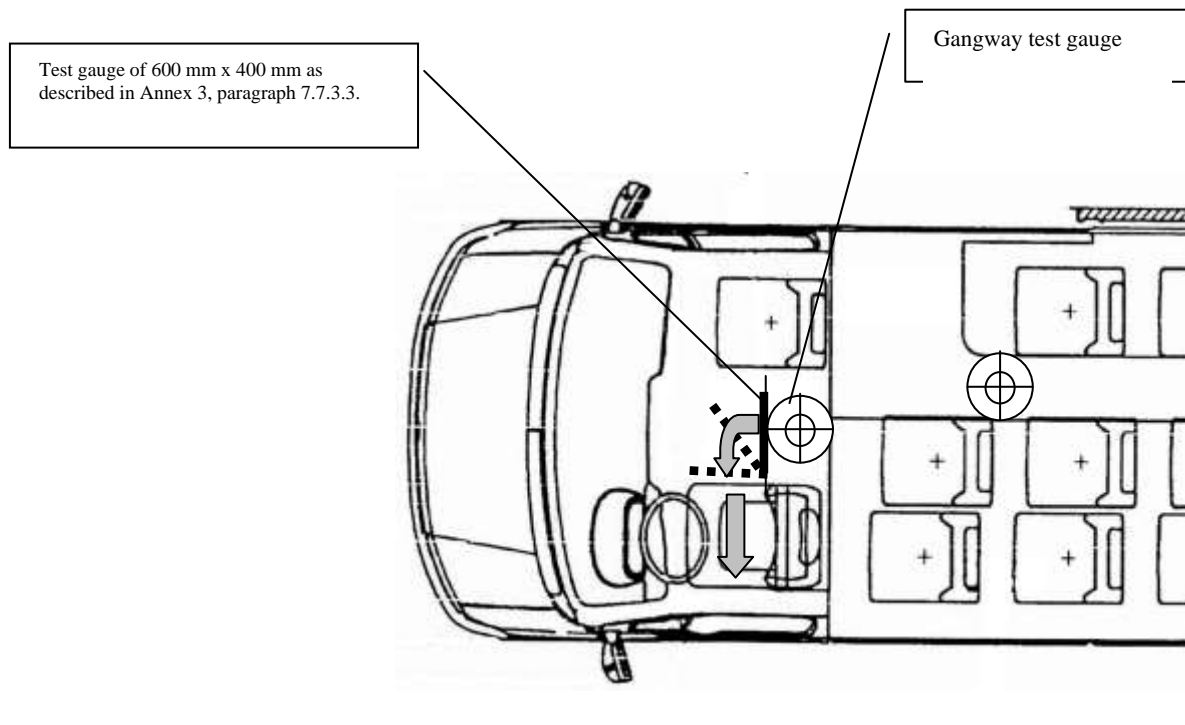
Figure 28 Access to driver's door (See Annex 3, paragraph 7.6.1.9.3.)
