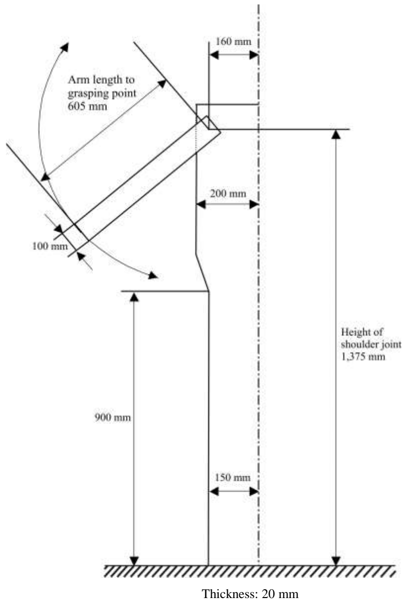
Figure 20 Testing device for positioning of handholds (See Annex 3, paragraph 7.11.2.1.)
