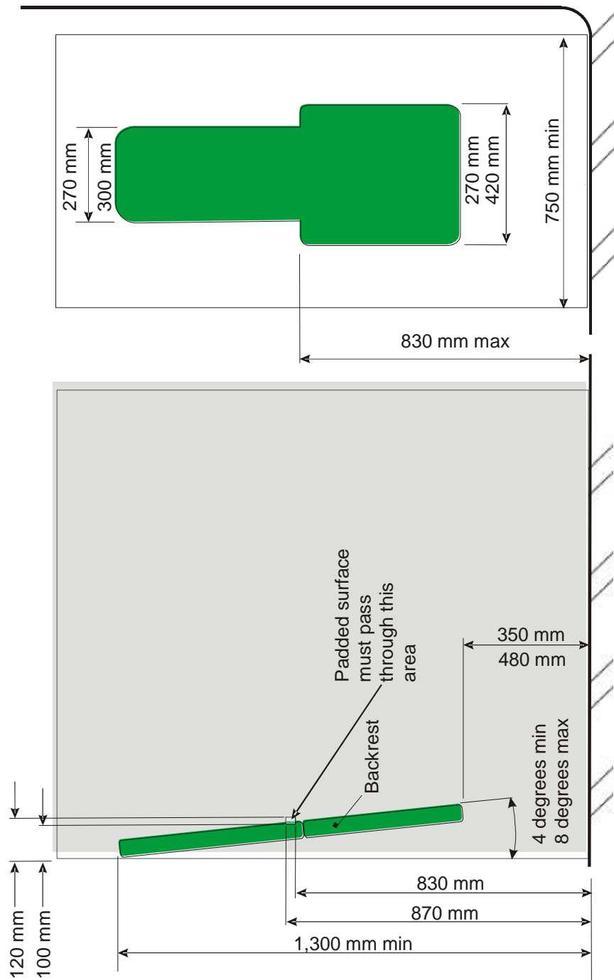
Figure 29 Example of a backrest for a rearward-facing wheelchair (See Annex 8, paragraph 3.8.6.)
