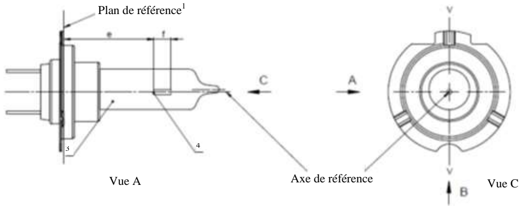
Figure 1 Dessin principal
