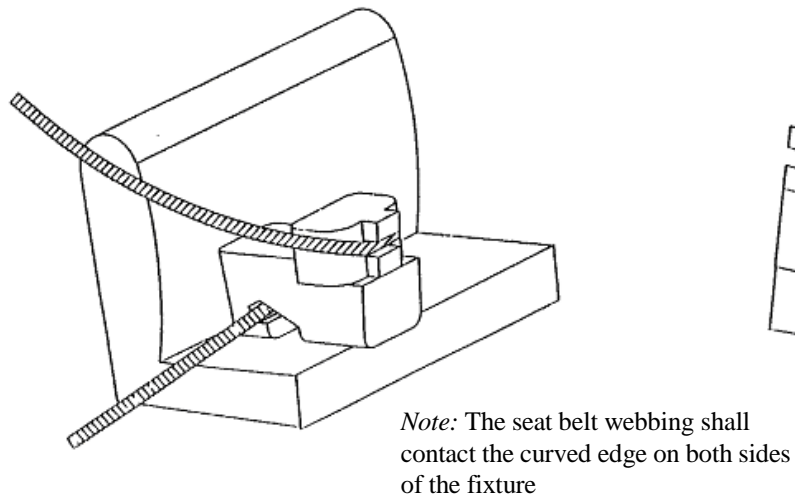
Figure 2 Installation of fixture onto vehicle seat (see paragraph 2.6.1.)
