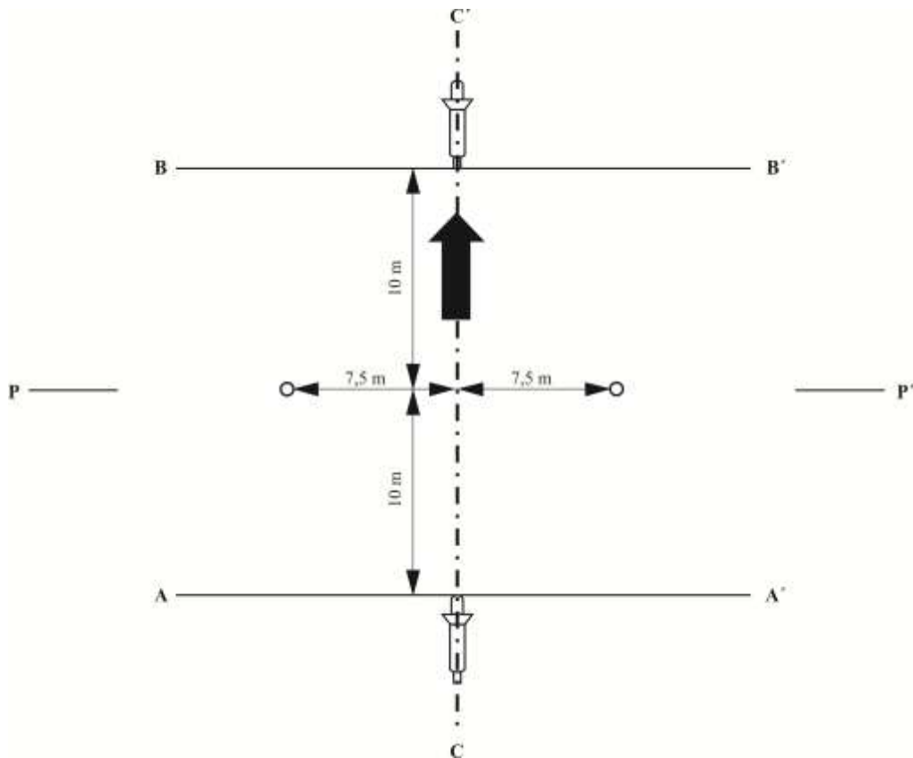
Figure 1 Measuring positions for vehicles in motion
