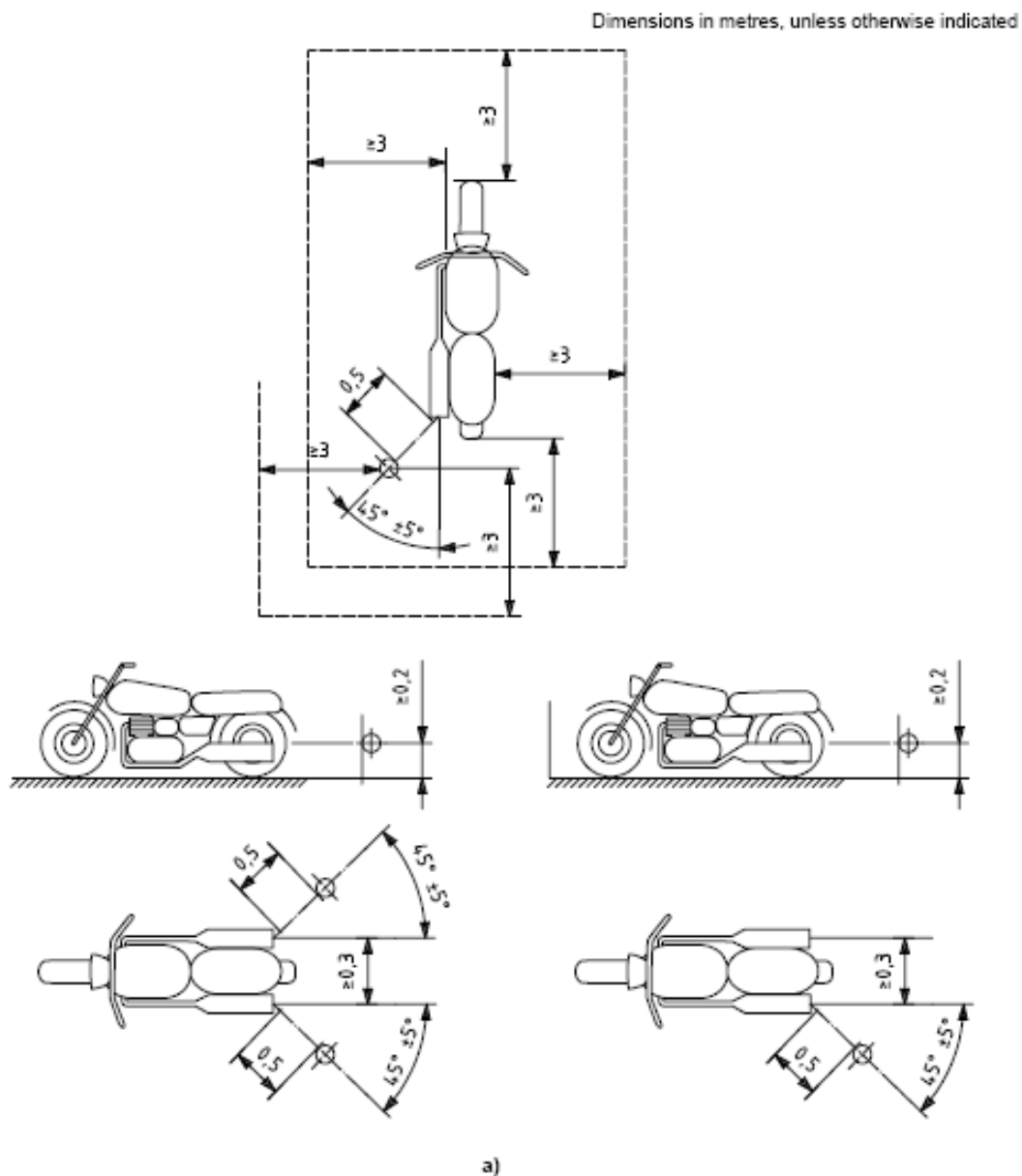
Figure 2 Measuring positions for stationary mopeds
