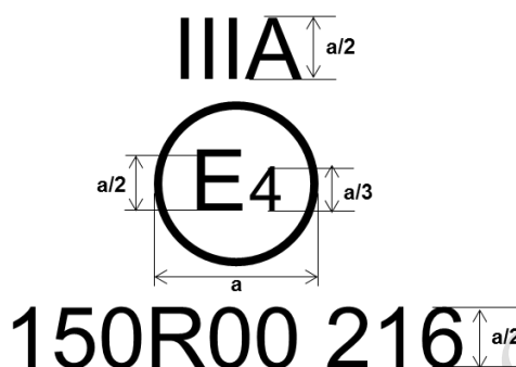
Figure A 24-I Marking examples for single devices
