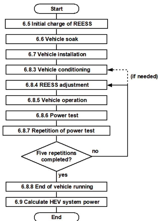
Figure 23 Test sequence
