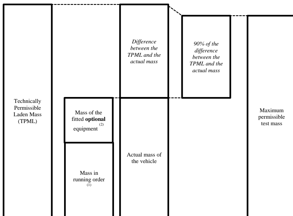
Figure 3 Mass definitions
