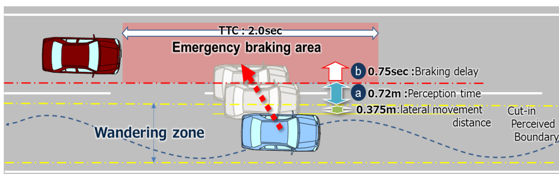
Driver model for the cut-in scenario
