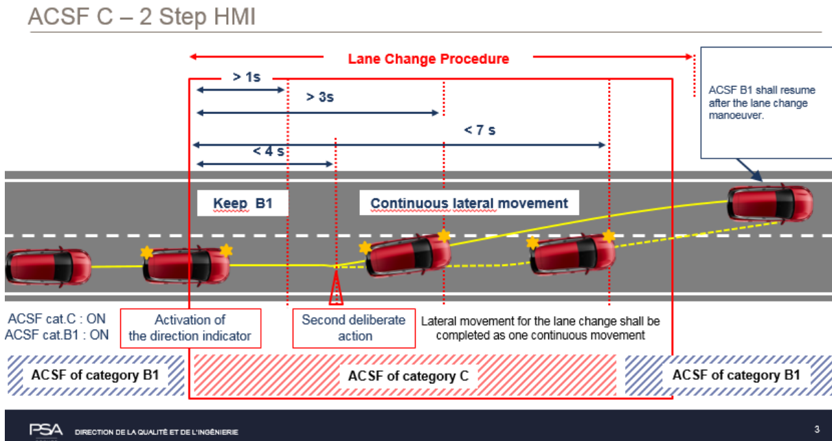
Description of the two-step HMI lane change procedure
