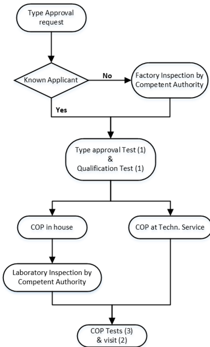
Type approval scheme (Flow chart)
