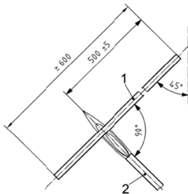
Figure 1 Apparatus for resistance to flame propagation (Dimensions in millimetres)
