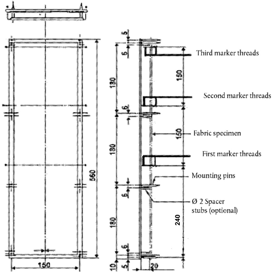
"Figure 1 Specimen holder (Dimensions in millimetres)
