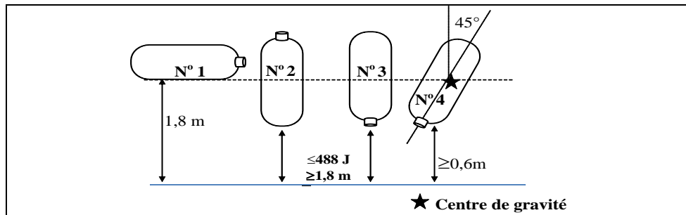
Figure 1 Orientations de chute
