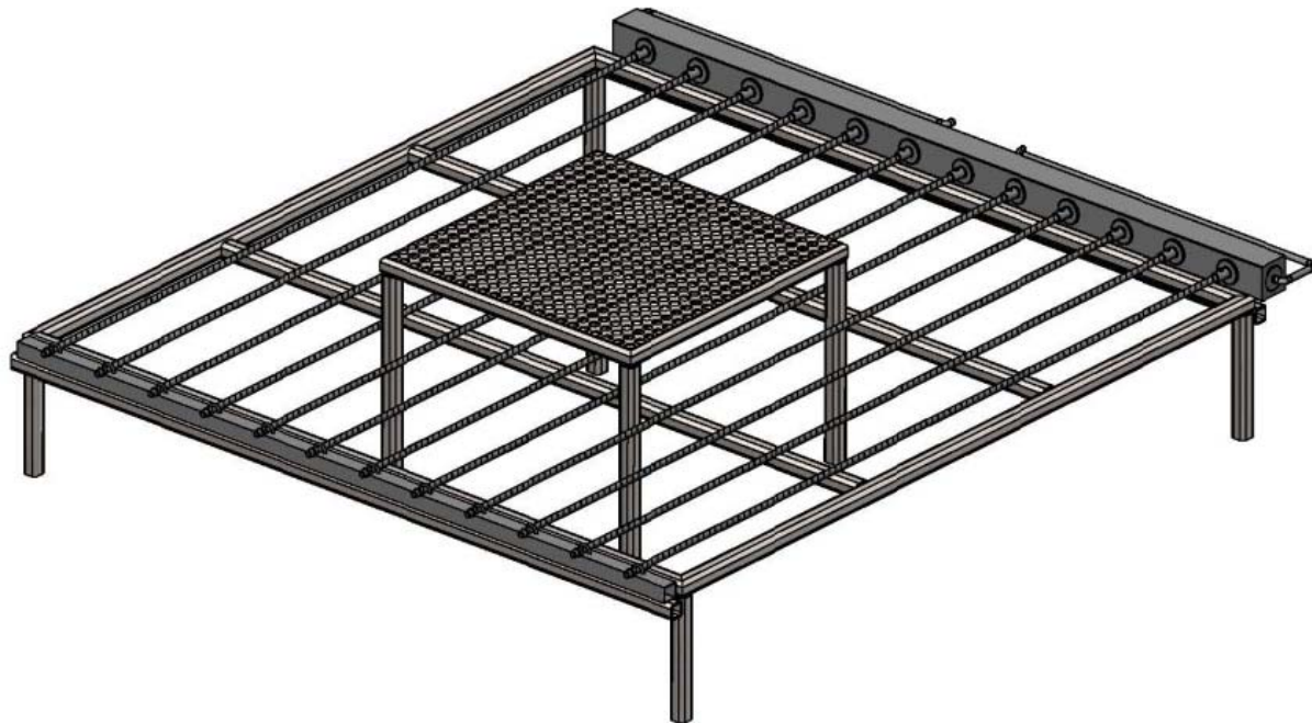
Figure 1: Proposed USA gas-fueled Test 6c burner assembly
