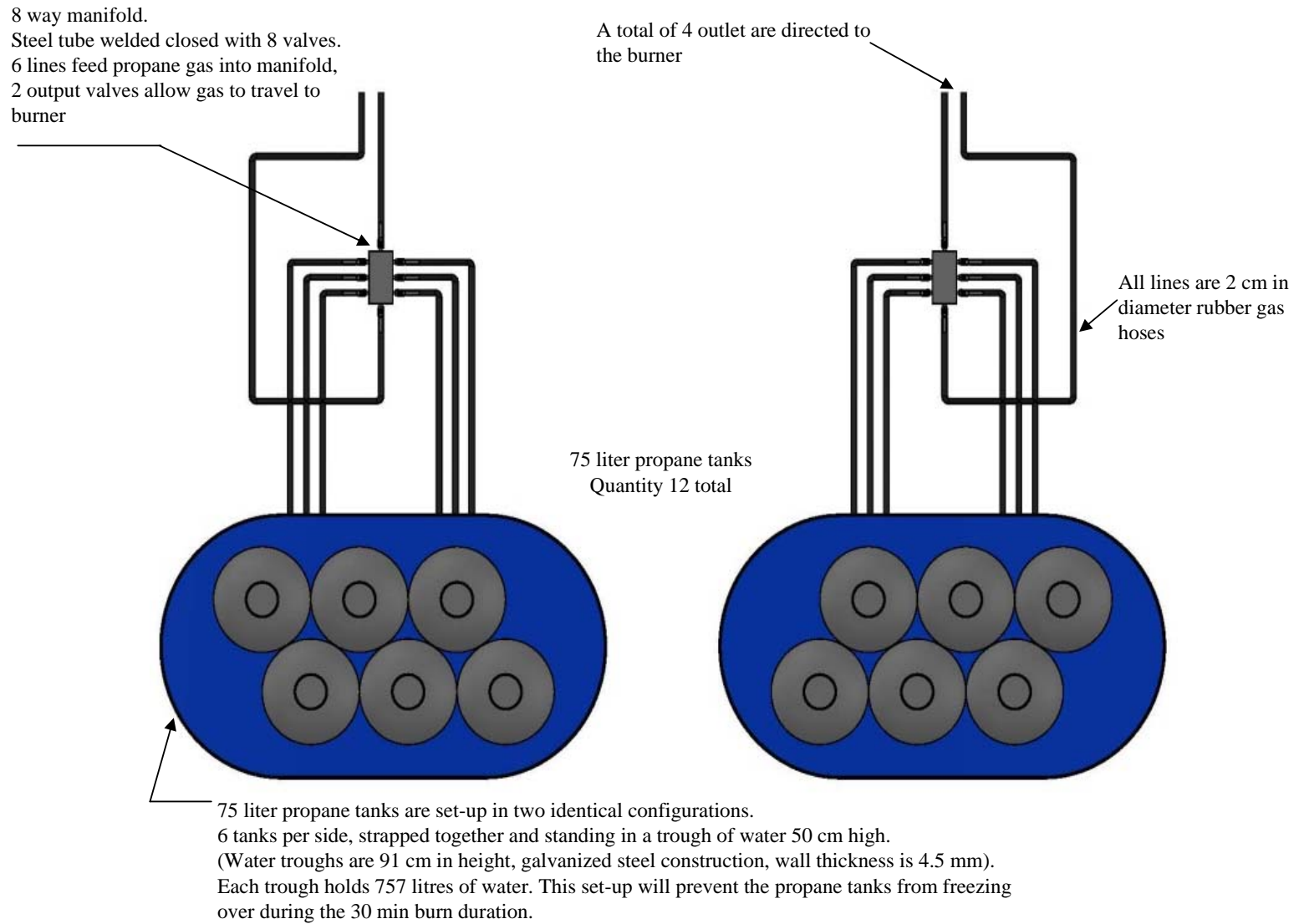
Figure 2: Proposed USA gas-fueled Test 6c
