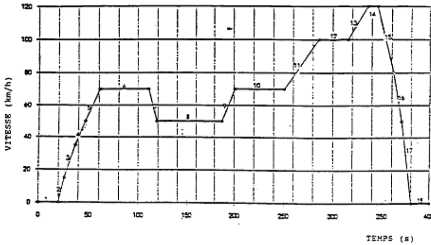
Cycle extra-urbain (400 s)
