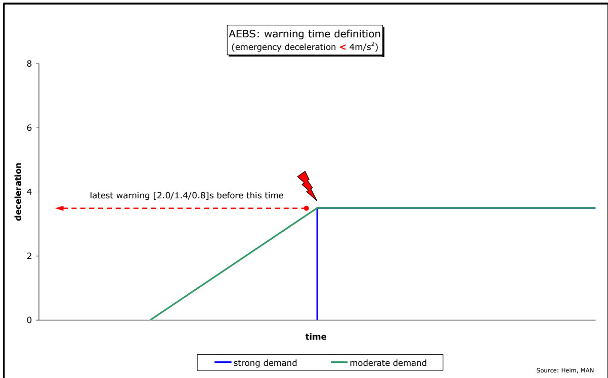
Figure 1: warning time at emergency braking demand < 4m/s 2
