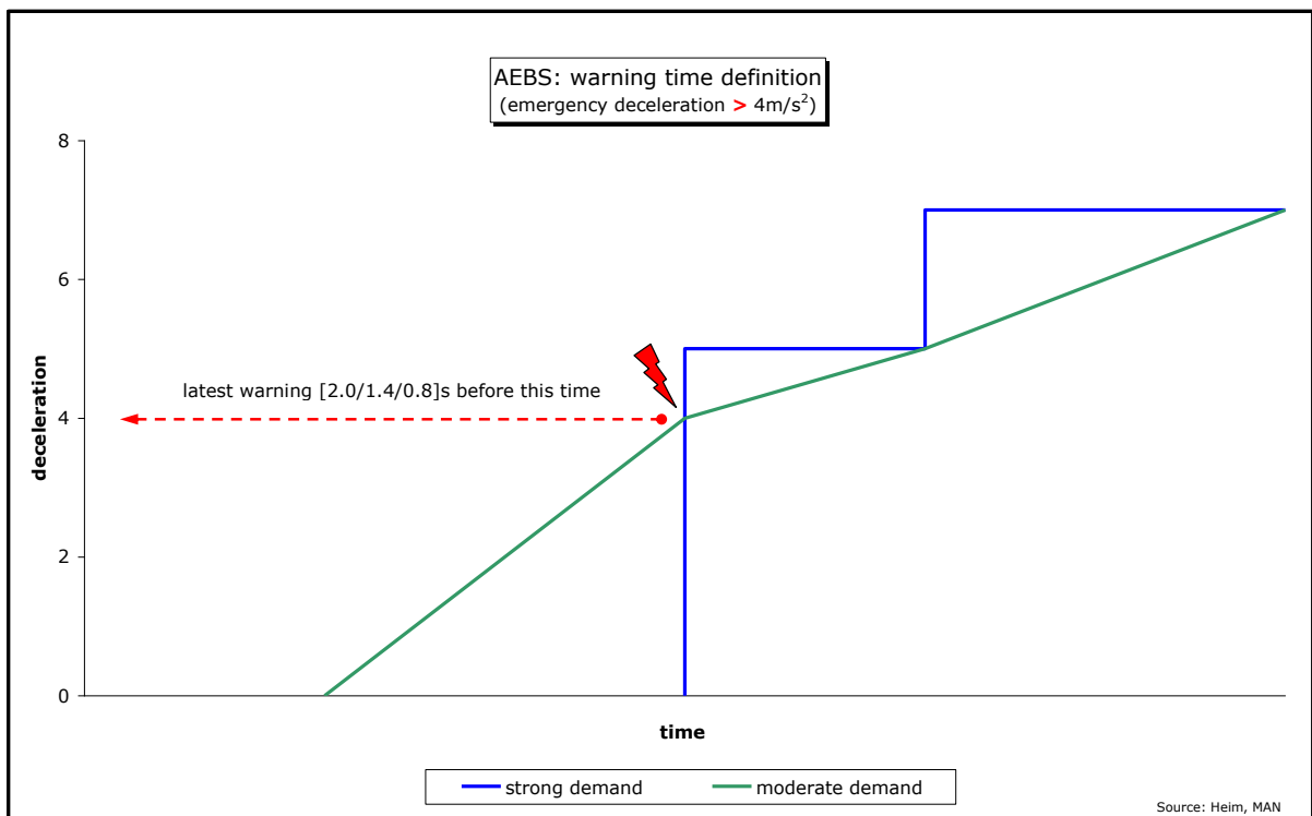
Figure 2: warning time at emergency braking demand > 4m/s 2
