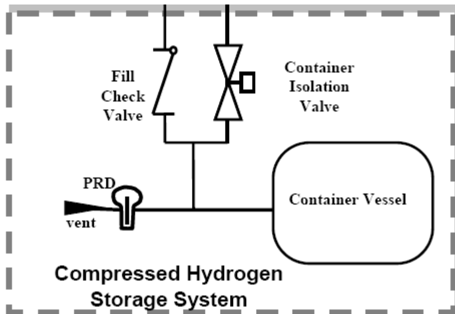
FIGURE 0 - HYPOTHETICAL COMPRESSED HYDROGEN STORAGE SYSTEM
