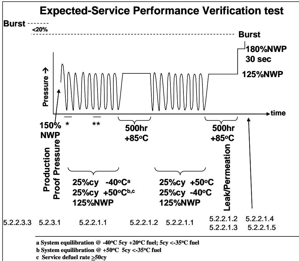
FIGURE 1 – COMPRESSED HYDROGEN STORAGE EXPECTED-SERVICE PERFORMANCE VERIFICATION TEST
