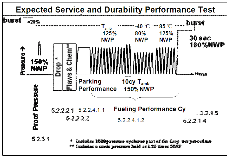
FIGURE 3 – COMPRESSED HYDROGEN STORAGE EXPECTED SERVICE AND DURABILITY TEST
