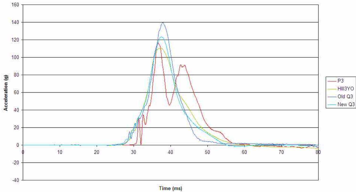
Head y-axis acceleration
