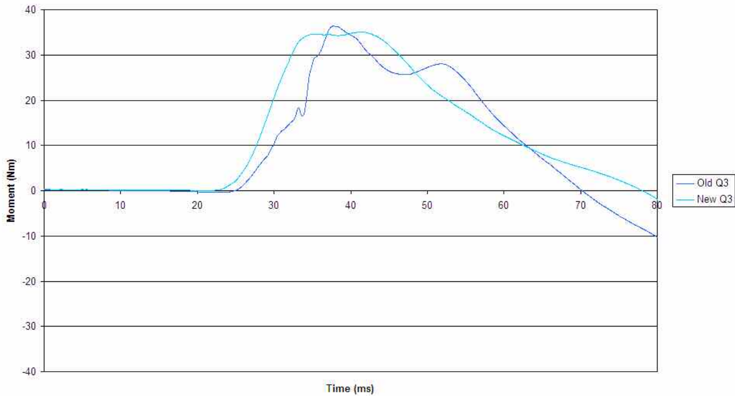
Lower neck x-axis moment
