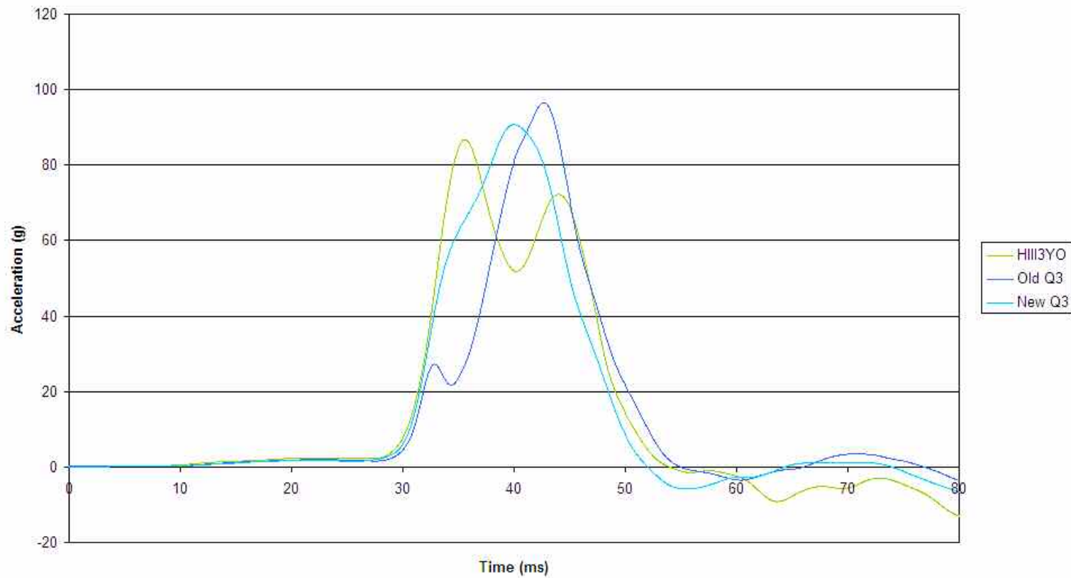
Pelvis y-axis acceleration
