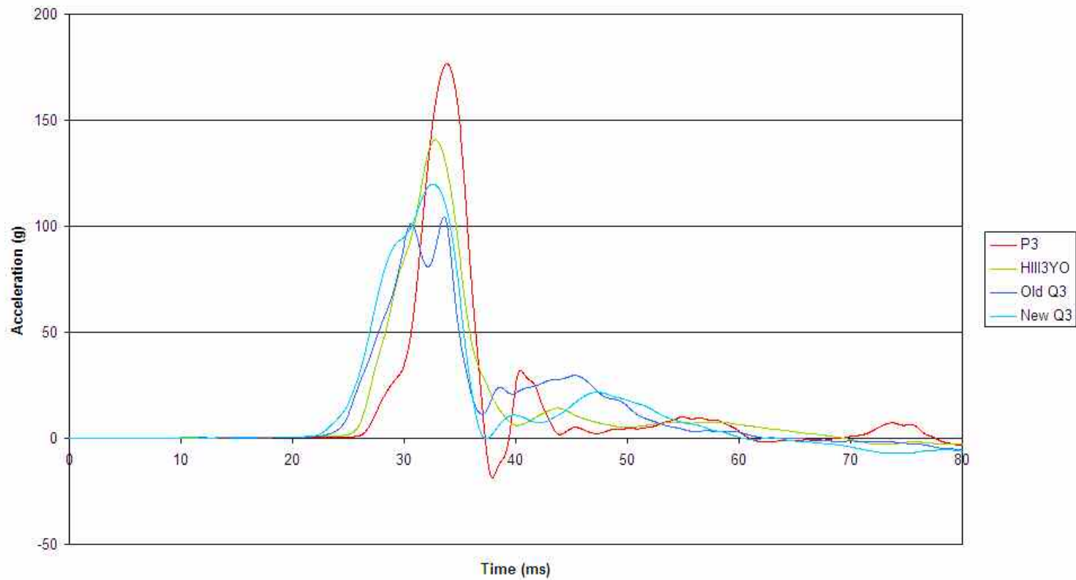
Chest y-axis acceleration
