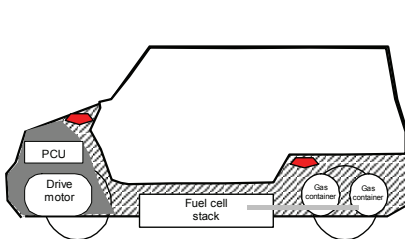
Example 3. Hydrogen system components installed under the floor of the body (two upward sections)
