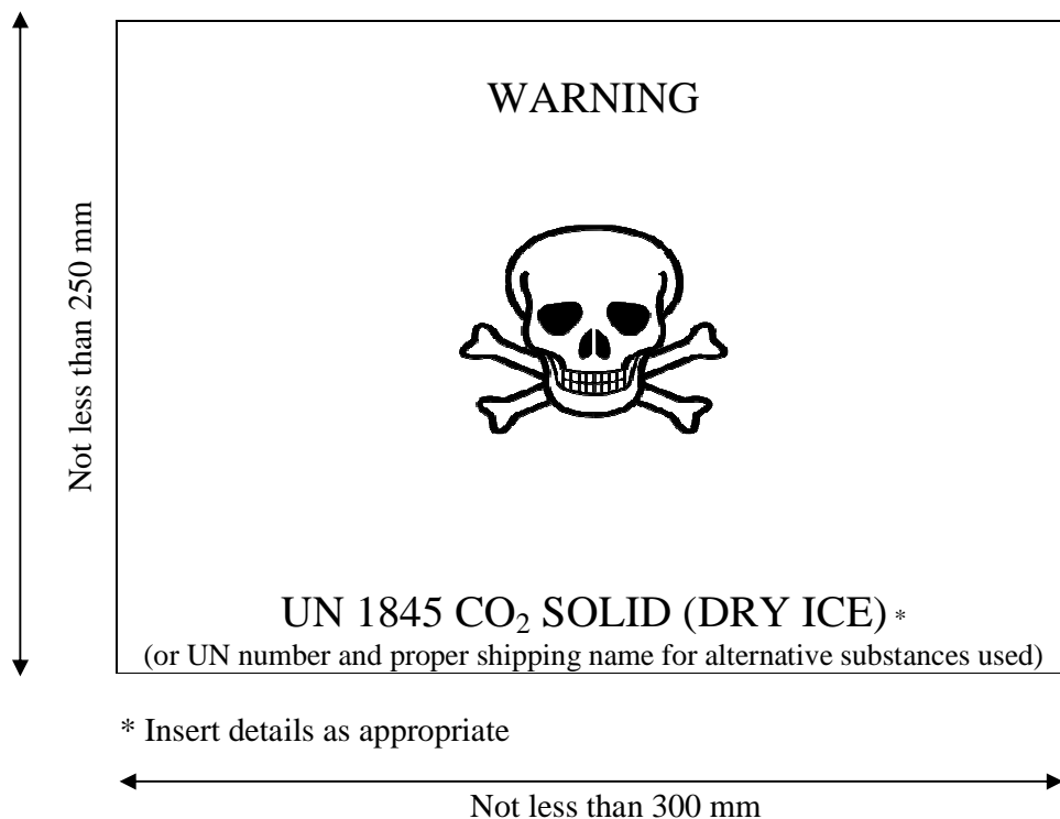
Figure 5.5.2: Cooling/conditioning warning sign
