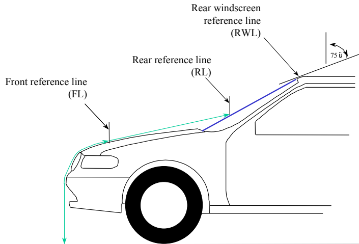
Figure 2A. Determination of FL, RL and RWL
