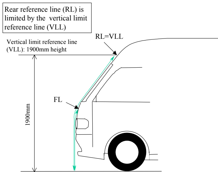
Figure 2C. Determination of FL, RL and VLL for tall cars
