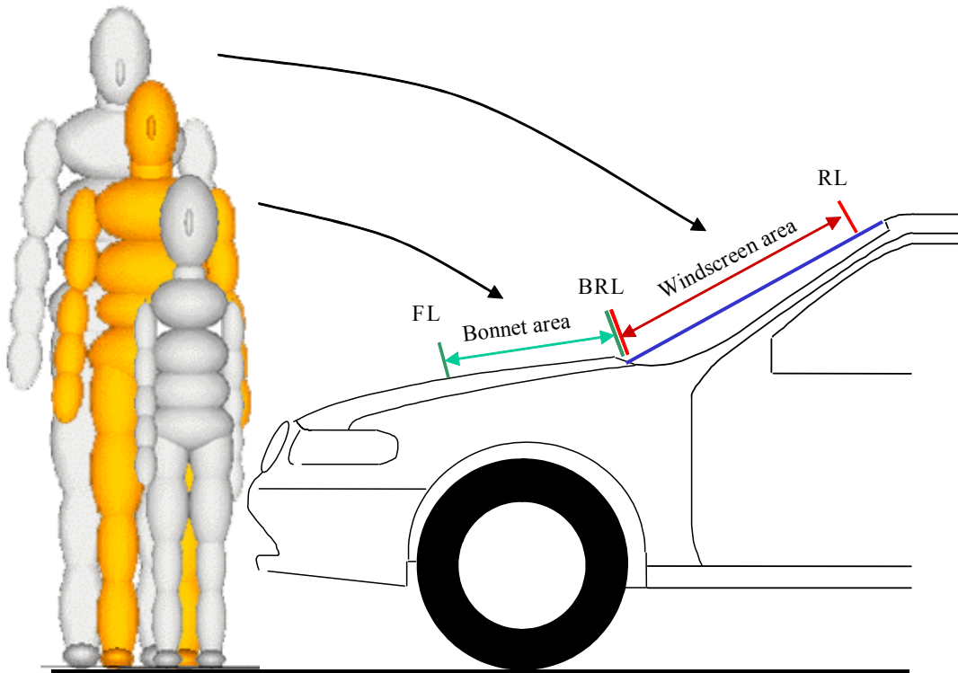
Figure 7. Principles of headform impact test
