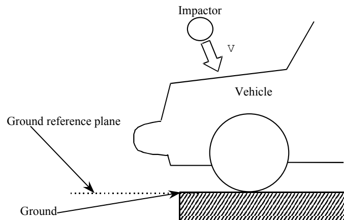
Figure 1: Configuration of IHRA Head Impact Test Procedure
