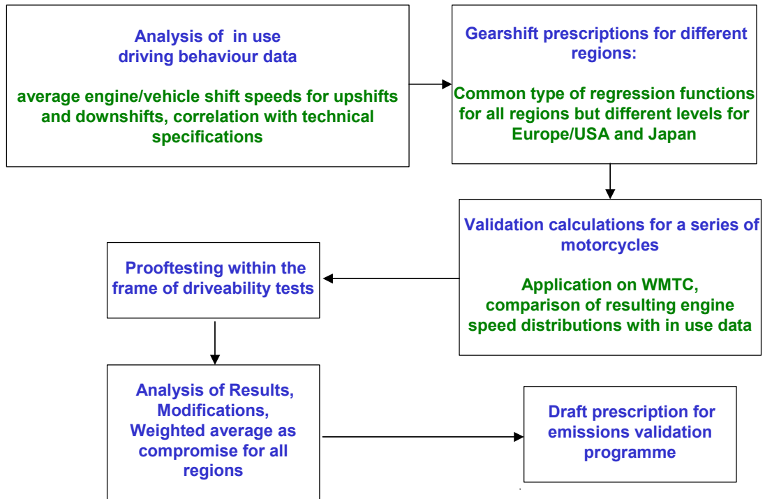
Figure 10: Flow chart of the gearshift prescription development
