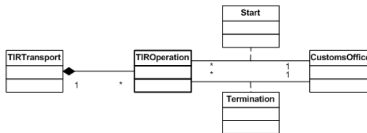
Figure 1.22 TIR operation class and its relationships
