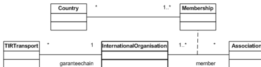
Figure 1.17 International organization class and its relationships
