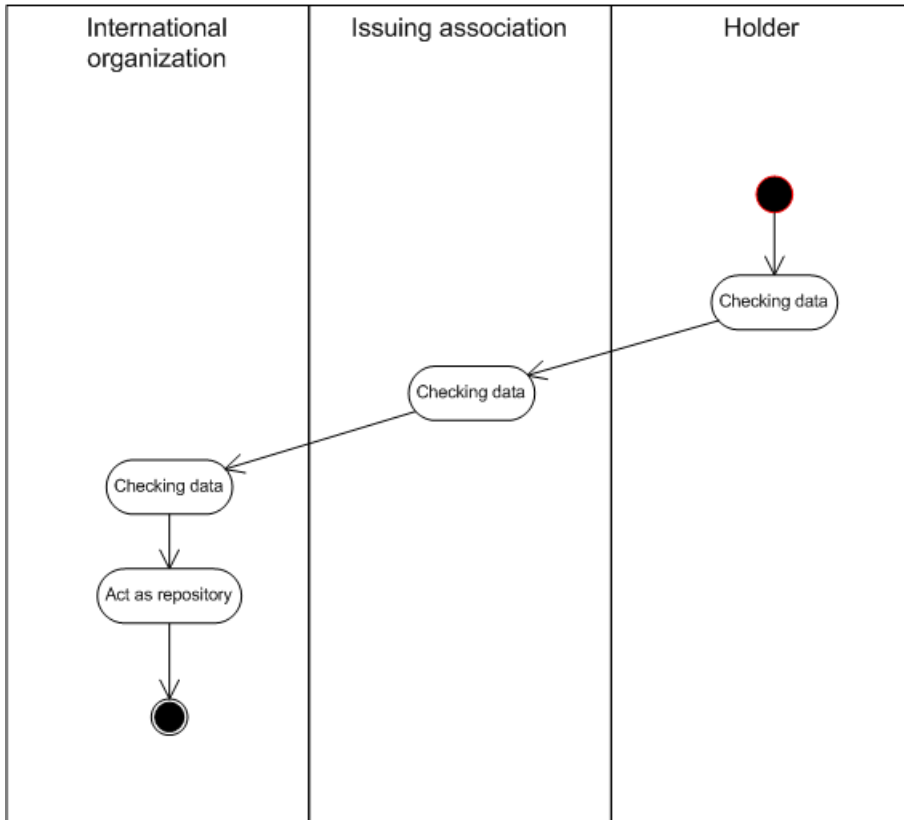
Figure 1.10 Return and repository activity diagram
