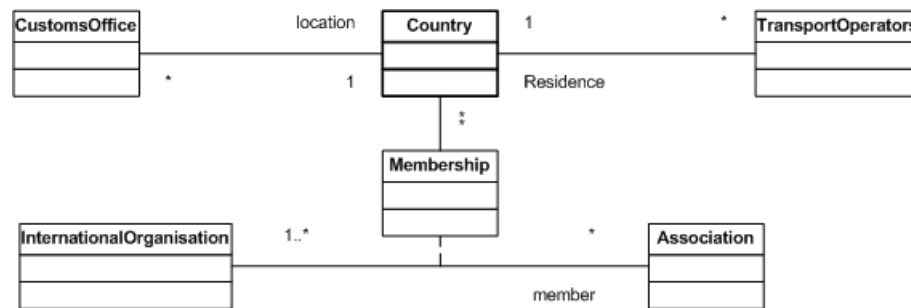
Figure 1.25 Country class and its relationships
