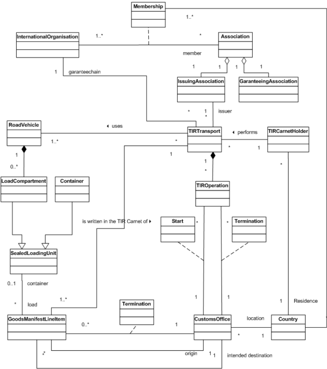
Figure 1.27 High-level class diagram
