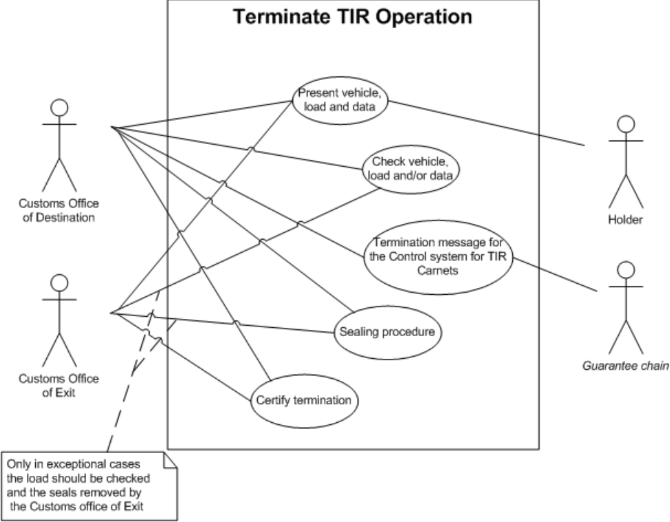
Figure 1.15 Terminate TIR operation use case diagram
