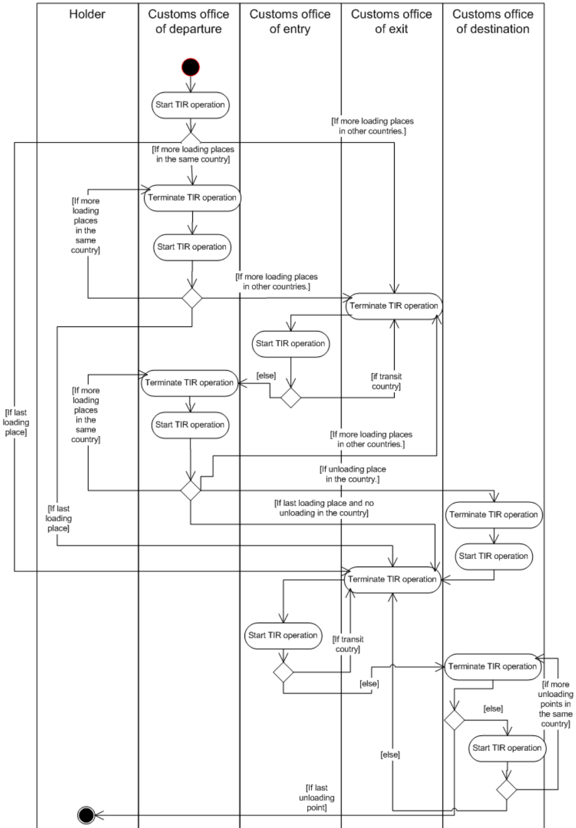
Figure 1.8 TIR transport activity diagram
