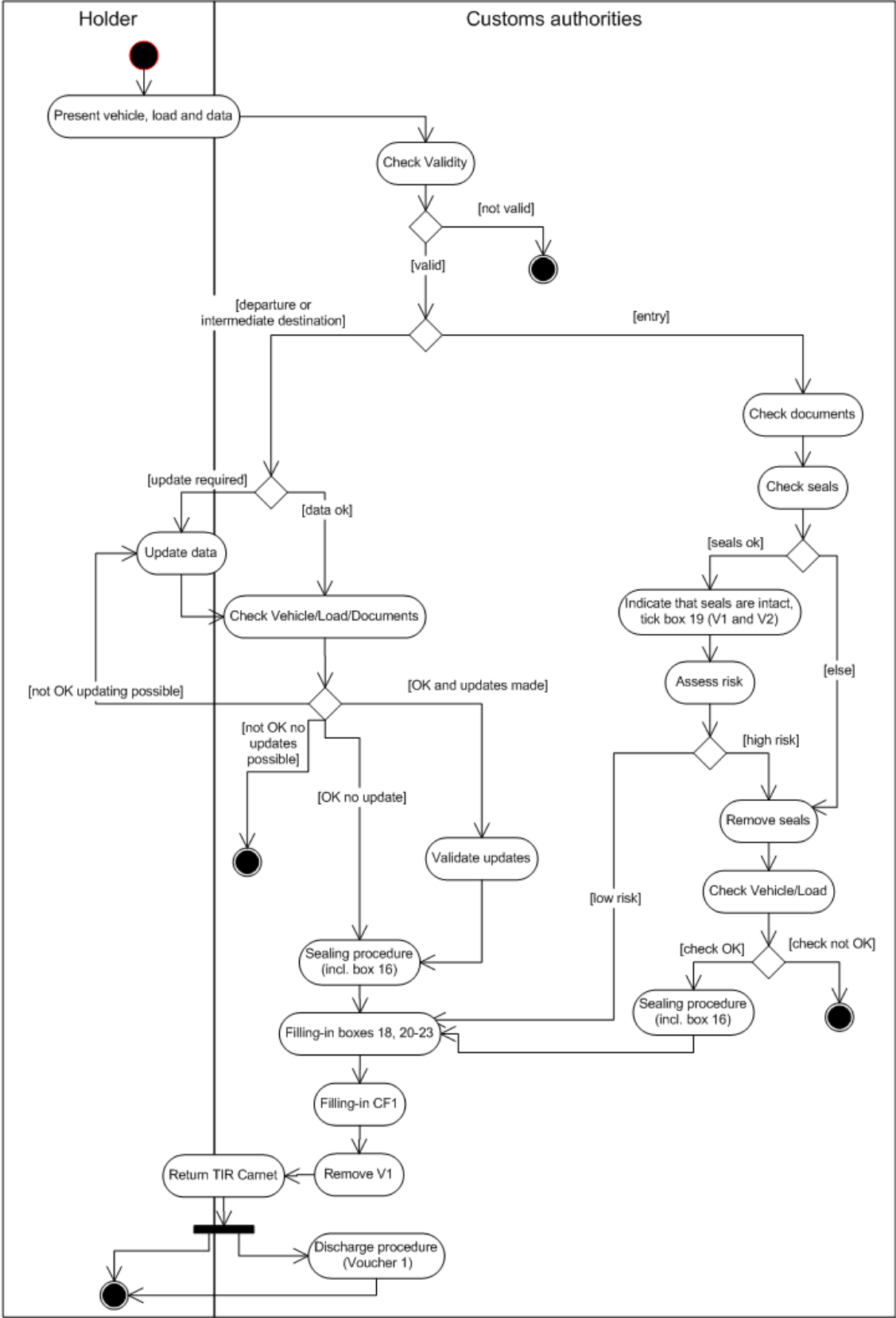
Figure 1.14 Start TIR operation activity diagram
