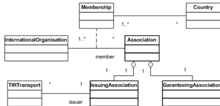
Figure 1.18 Association class and its relationships
