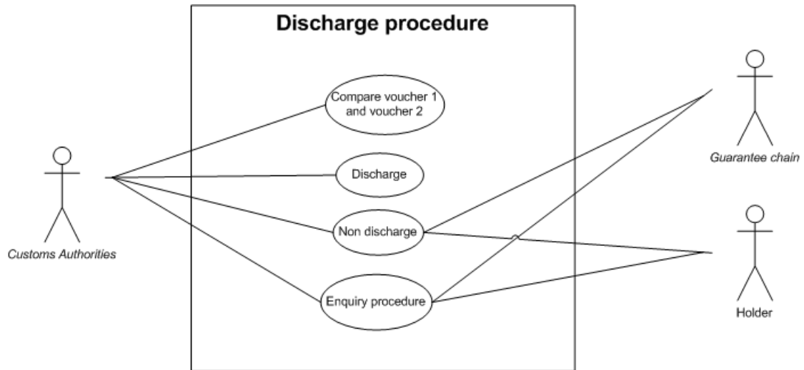
Figure 1.11 Discharge procedure use case diagram
