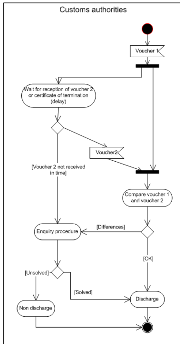
Figure 1.12 Discharge procedure activity diagram
