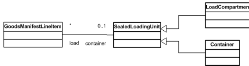
Figure 1.20 Sealed loading unit class and its relationships
