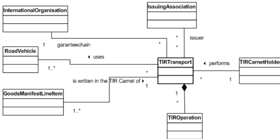
Figure 1.21 TIR transport class and its relationships
