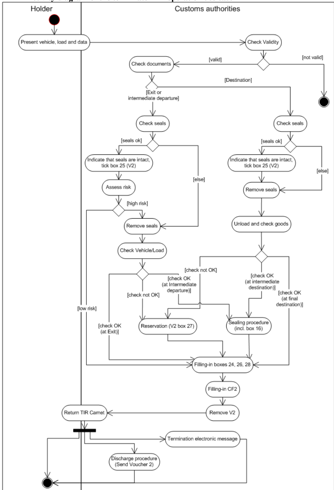
Figure 1.16 Terminate TIR operation activity diagram
