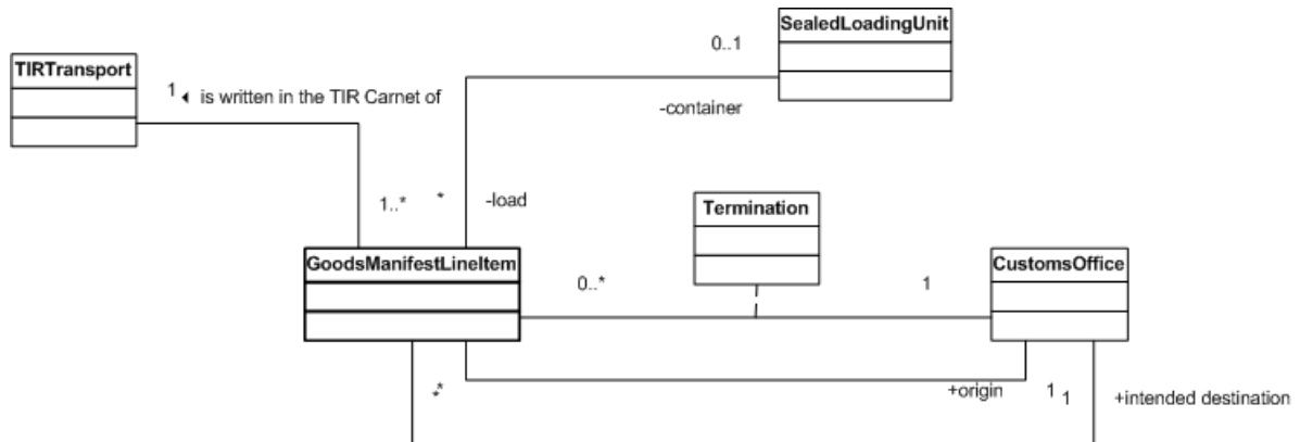
Figure 1.23 Goods Manifest Line Item class and its relationships
