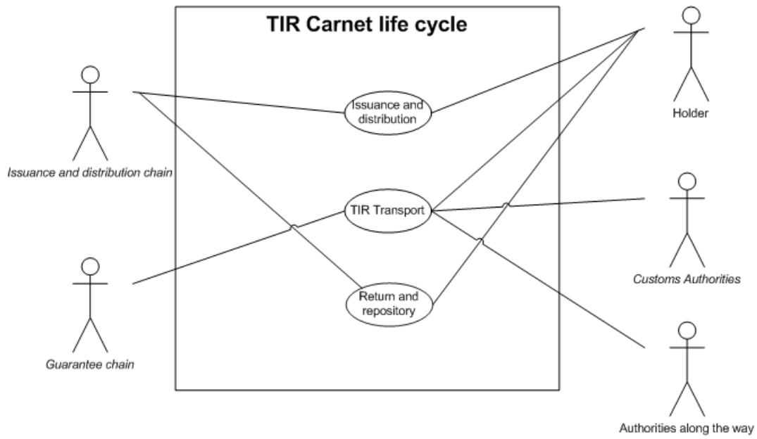
Figure 1.3 TIR Carnet life cycle use case diagram
