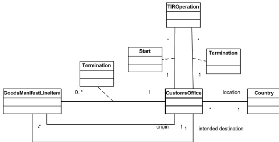
Figure 1.24 Customs office class and its relationships
