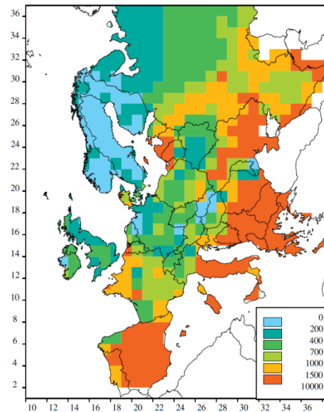
Figure 2.5: The 2-percentile critical load for acidification (CL max ) (equivalents/ha/year)
