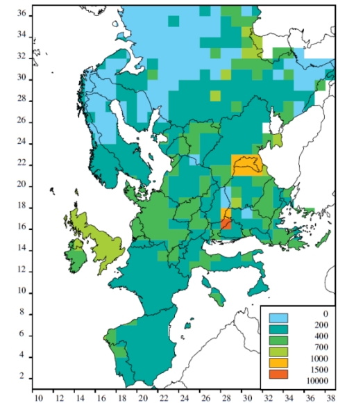
Figure 2.6: The 2-percentile critical load for eutrophication (equivalents/ha/year)
