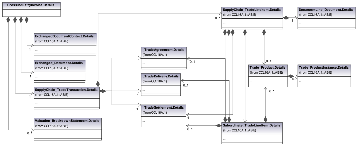
190 Figure 2.5.1. Cross Industry Invoice conceptual data model
