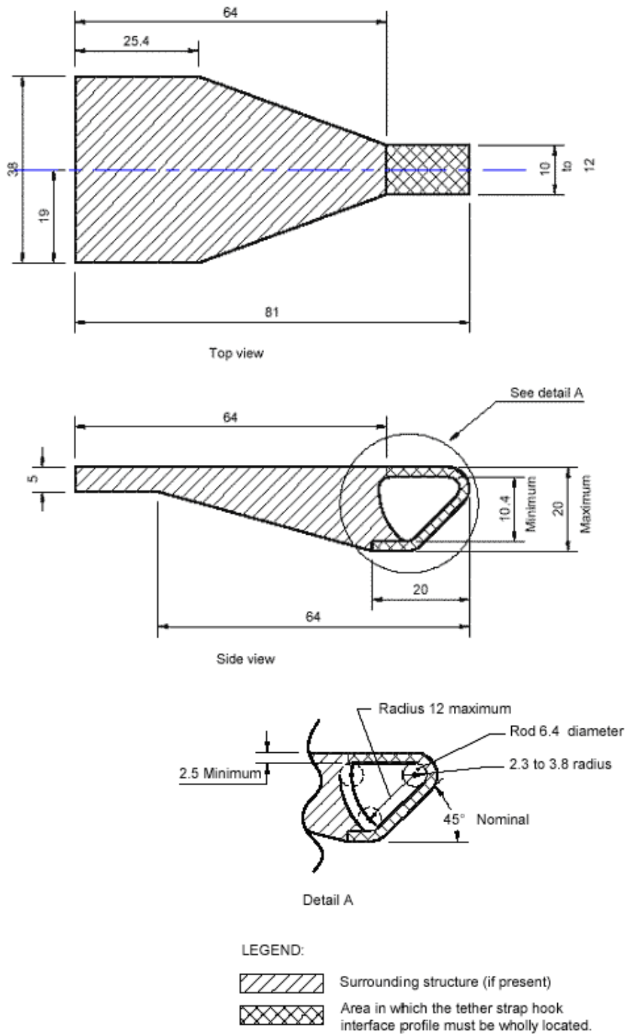
Figure 3: ISOFIX Top tether connector (hook type) dimensions
