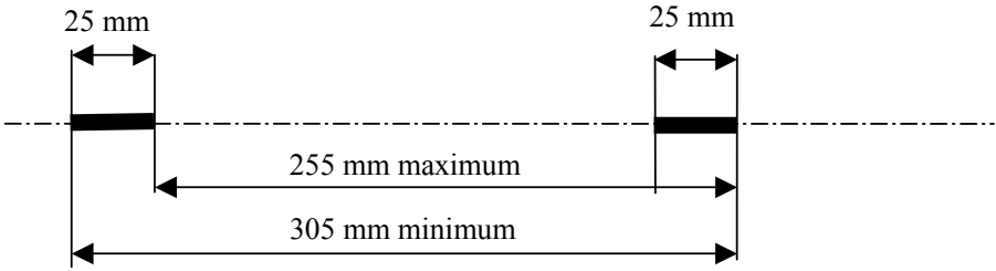
Figure 4: Distance between both low anchorage zones
