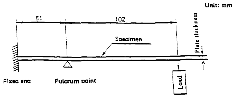
Figure 21 : Method of setting up the test specimen
