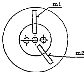
FIGURE 2a: Containers with circumferential welds only and side-mounted valve blocks; Location of test-pieces
