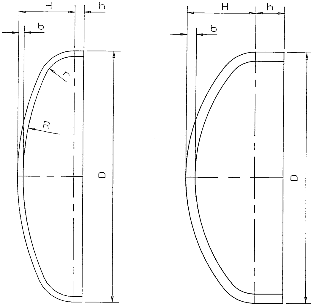
torispherical ends
