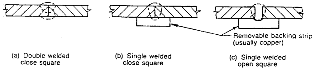
types of main longitudinal butt welds
