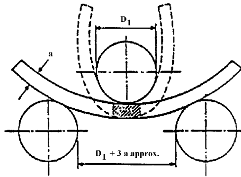
FIGURE 1 ILLUSTRATION OF BEND TEST
