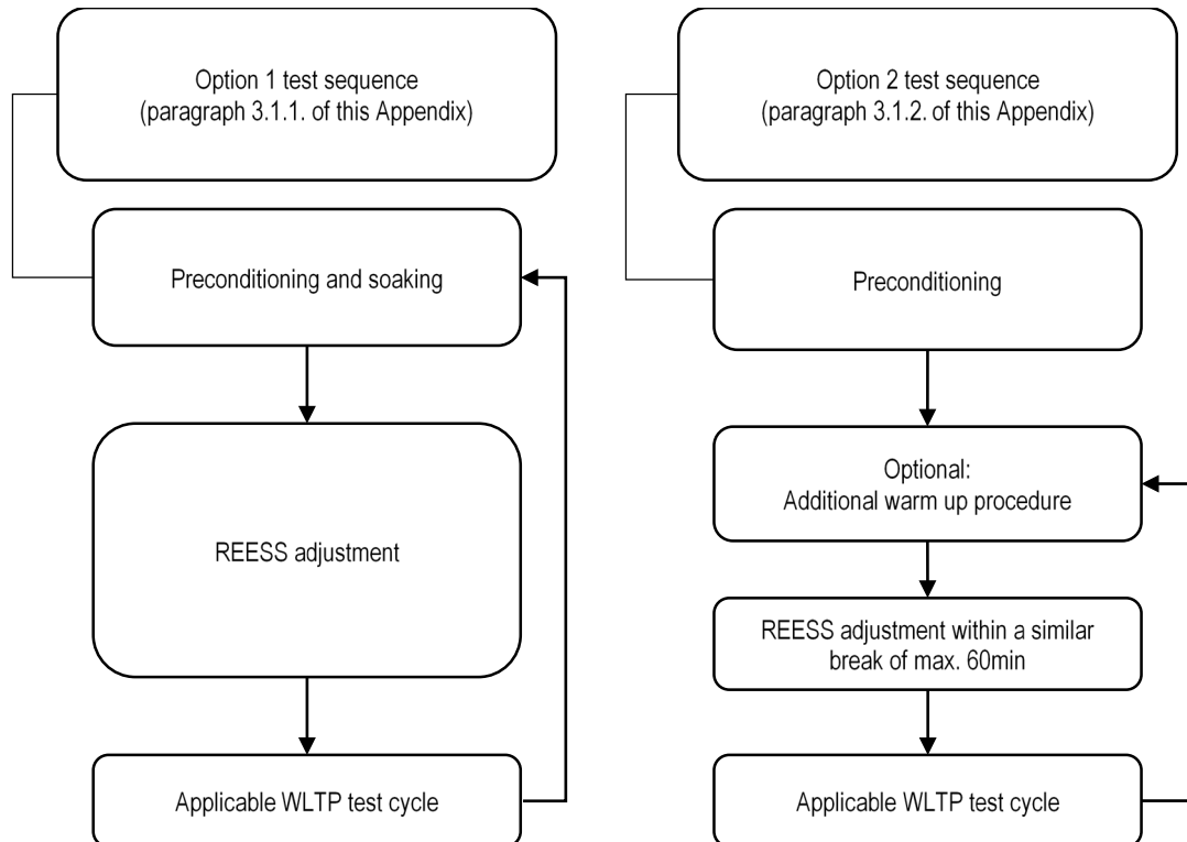
Figure A8.App2/1 OVC-HEV test sequences
