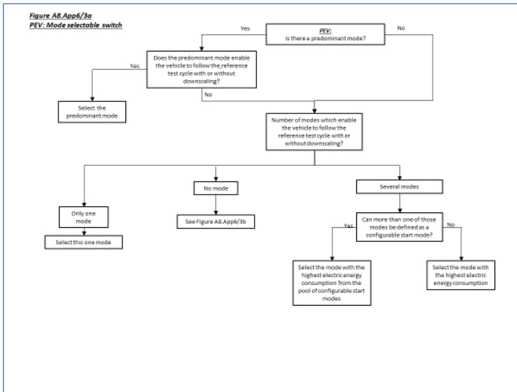
Figure A8.App6/3a and Figure A8.App6/3b Selection of the driver-selectable mode for PEVs
