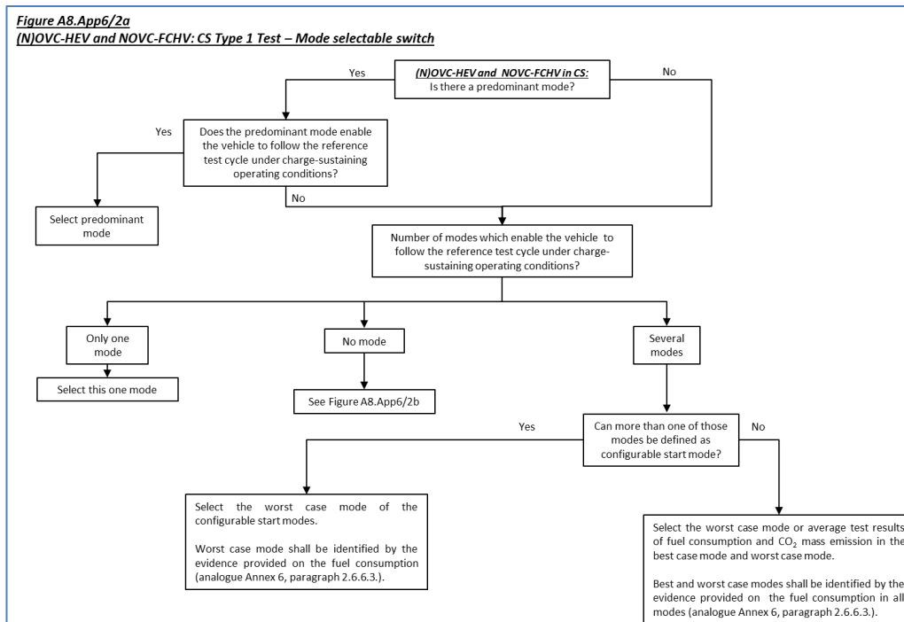
Figure A8.App6/2a and Figure A8.App6/2b Selection of a driver-selectable mode for OVC-HEVs, NOVC-HEVs and NOVC-FCHVs under charge-sustaining operating condition
