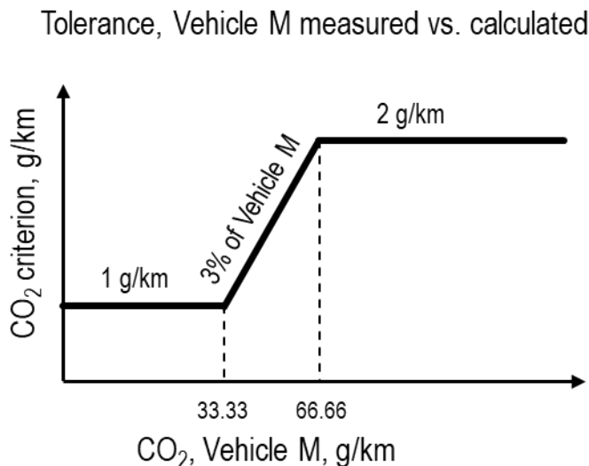
Figure A8/6 Linearity criterion for vehicle M
