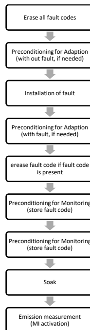
Figure C5.App1/1 Overview of demonstration test
