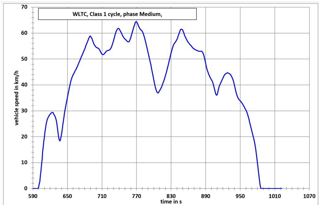
Figure A1/2a WLTC, Class 1 cycle, phase Medium 1
