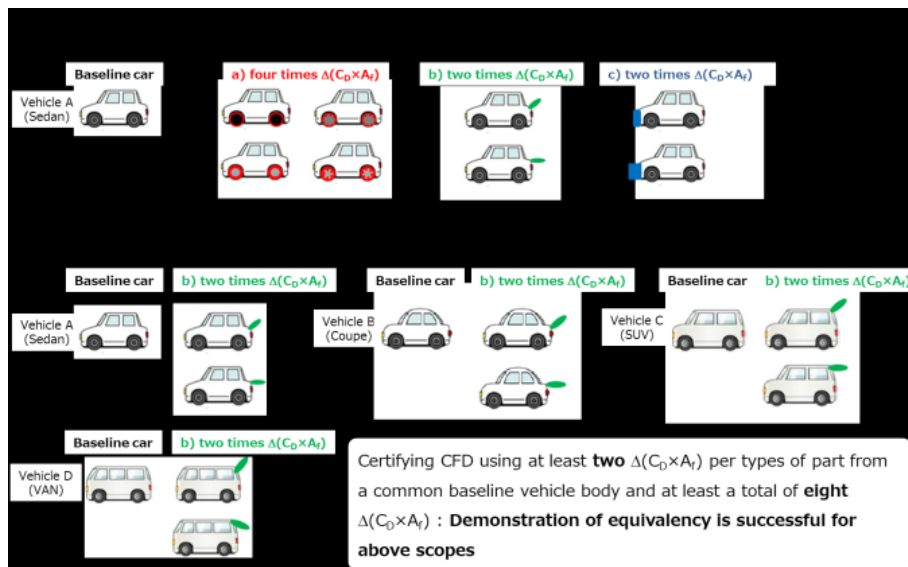
Figure A7/1 Example of application of the alternative method for determination of aerodynamic influence of optional equipment
