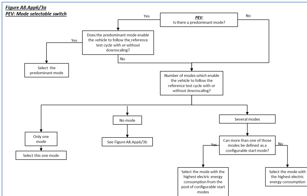
Figure A8.App6/3a and Figure A8.App6/3b Selection of the driver-selectable mode for PEVs
