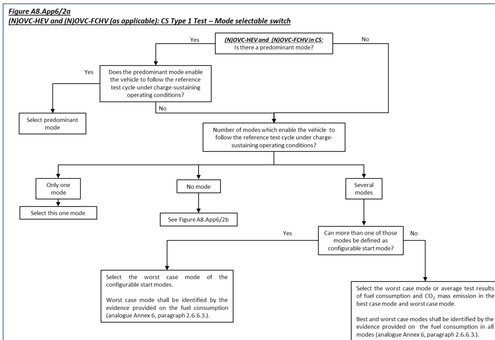
Figure A8.App6/2a and Figure A8.App6/2b Selection of a driver-selectable mode for OVC-HEVs, NOVC-HEVs, OVC-FCHVs and NOVC-FCHVs under charge-sustaining operating condition
