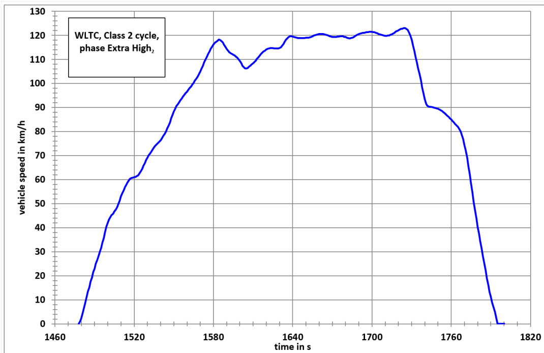
Figure A1/6 This figure is only applicable for Level 1A WLTC, Class 2 cycle, phase Extra High 2
