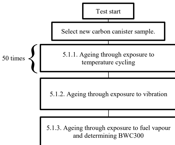
Figure C3/1 Carbon canister bench ageing procedure
