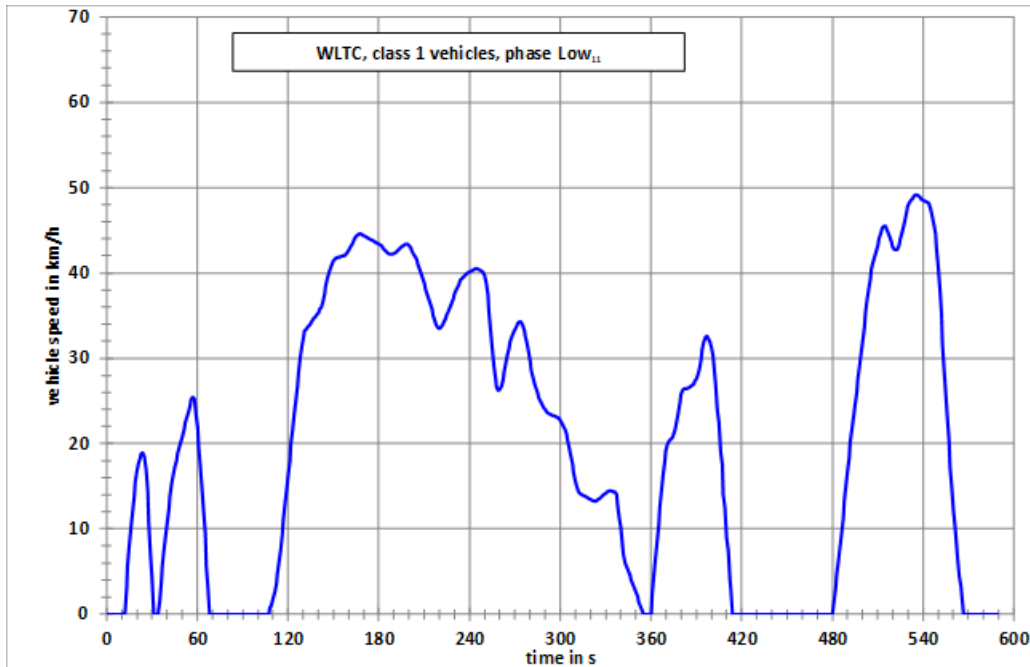
WLTC, Class 1 cycle, phase Low 11
