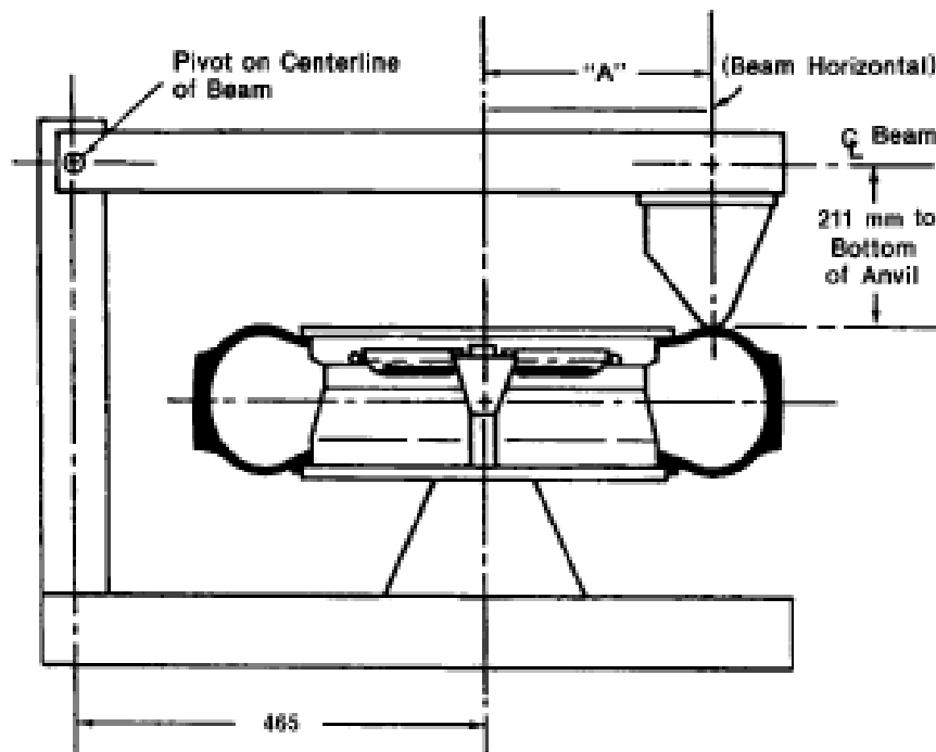
Bead Unseating Fixture (all dimension in mm) and table of "A" dimensions
