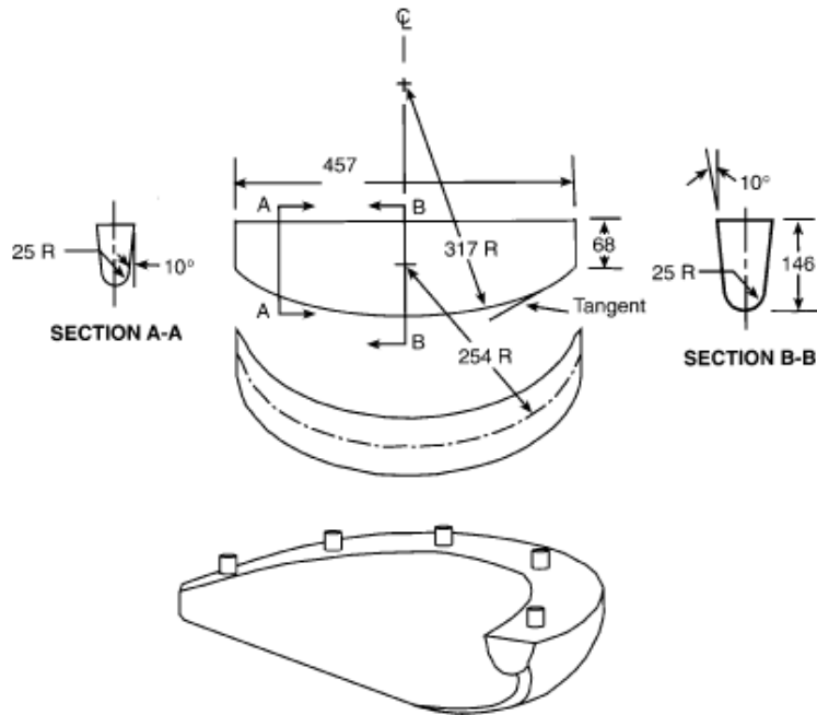
Diagram of bead unseating block (all dimensions in mm)
