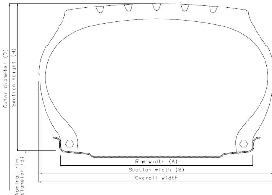
Drawing of a normal tyre showing various dimensions
