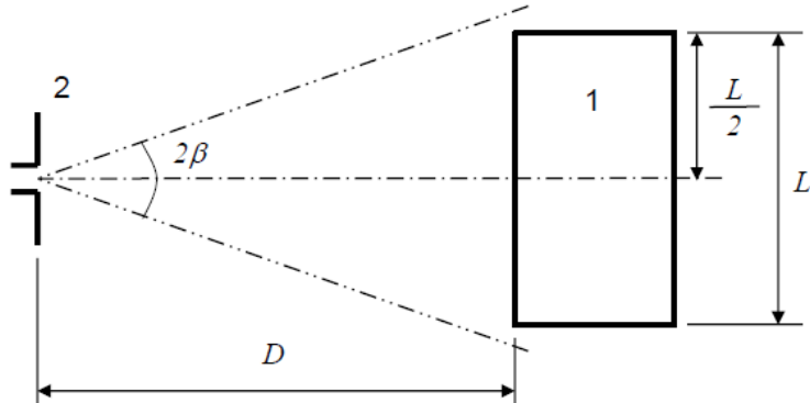
Figure 4 Antenna position for N = 1 (one antenna position to be used) – Horizontal polarization shown
