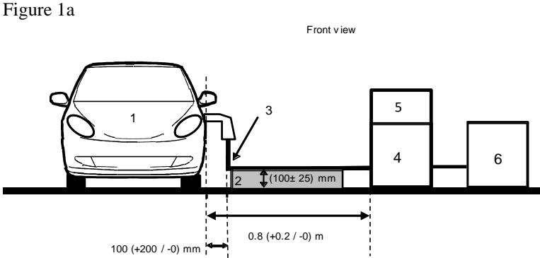
Figure 1 Vehicle in configuration "REESS charging mode coupled to the power grid" Example of test setup for vehicle with plug located on vehicle side
