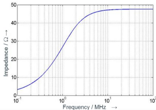
Figure 2 Characteristics of the AN impedance Z_{PB}
