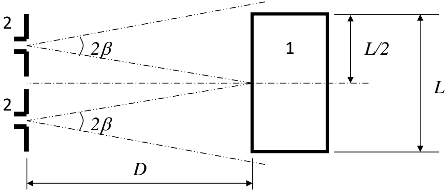
Figure 5 Antenna positions for N = 2 (multiple antenna positions to be used) – Horizontal polarization shown
