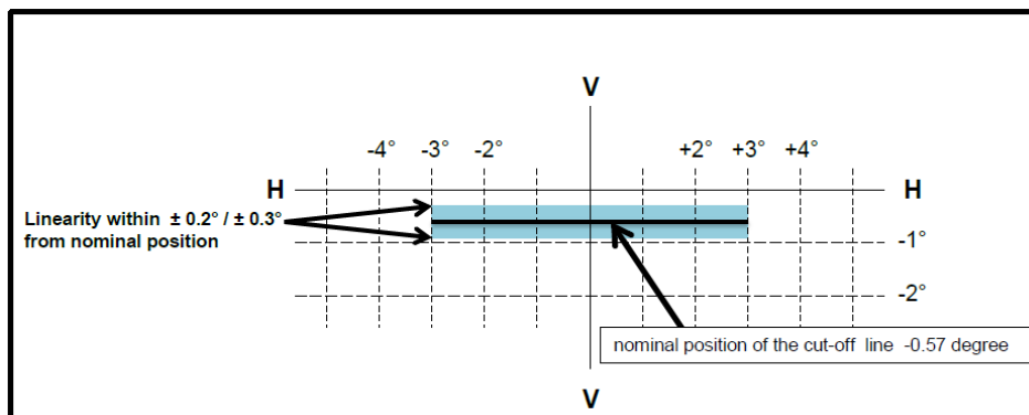
Shape and position of the "cut-off" line of symmetrical passing-beam headlamp
