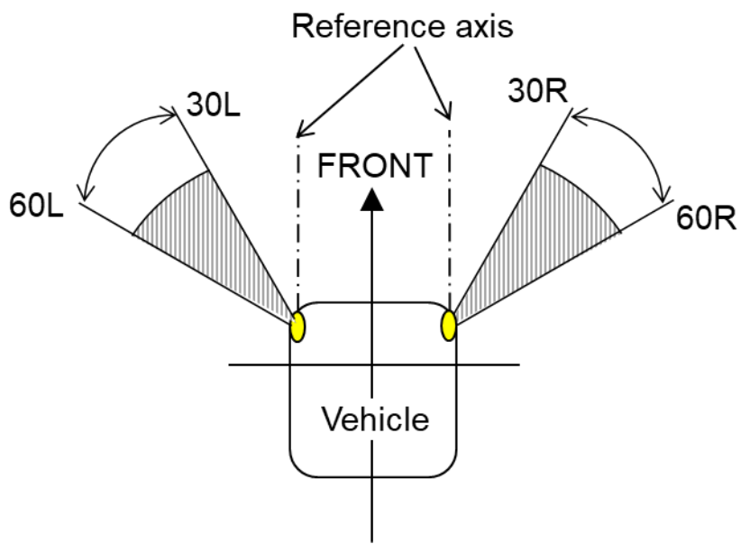
Figure A4-XIII Horizontal geometric visibility for cornering lamps
