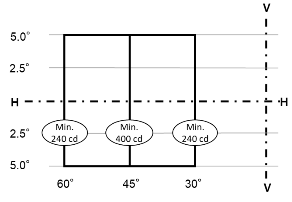
Figure A4-XII Measuring points for cornering lamps (left side lamp)
