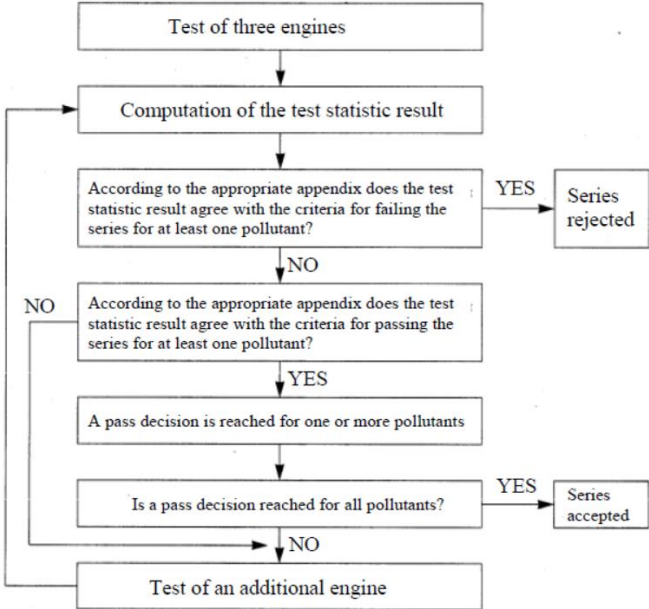
Figure 4. Schematic flow of production conformity testing
