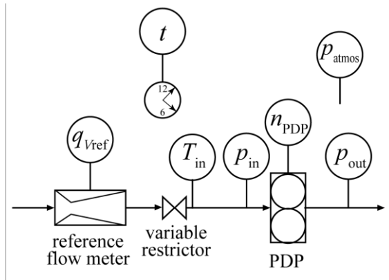
Figure A.4-4 Schematic diagrams for diluted exhaust flow CVS calibration
