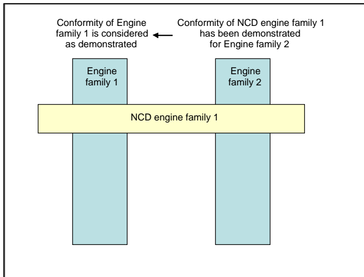
Figure A.9-3. Previously demonstrated conformity of an NCD engine family
