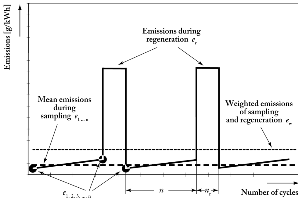
Figure A.4-1. Scheme of infrequent regeneration with n number of measurements and n_r number of measurements during regeneration
