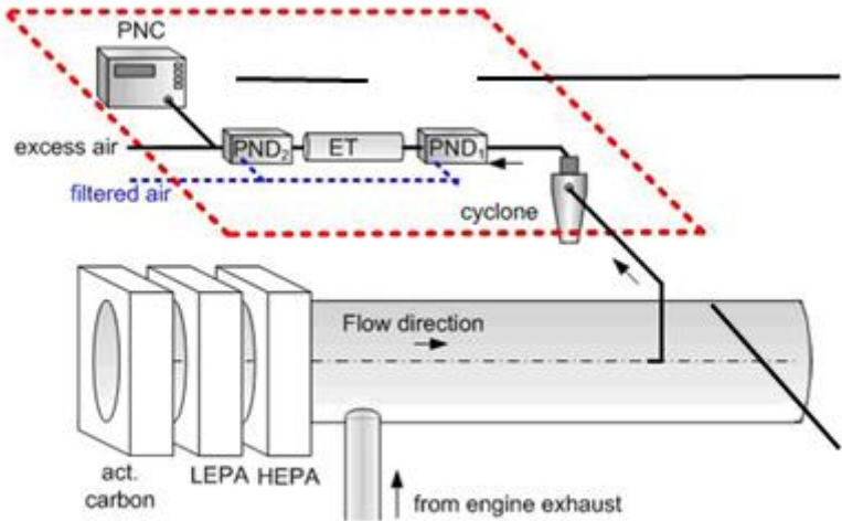
Figure A.4-9. Schematic of recommended particle sampling system – Full flow sampling
