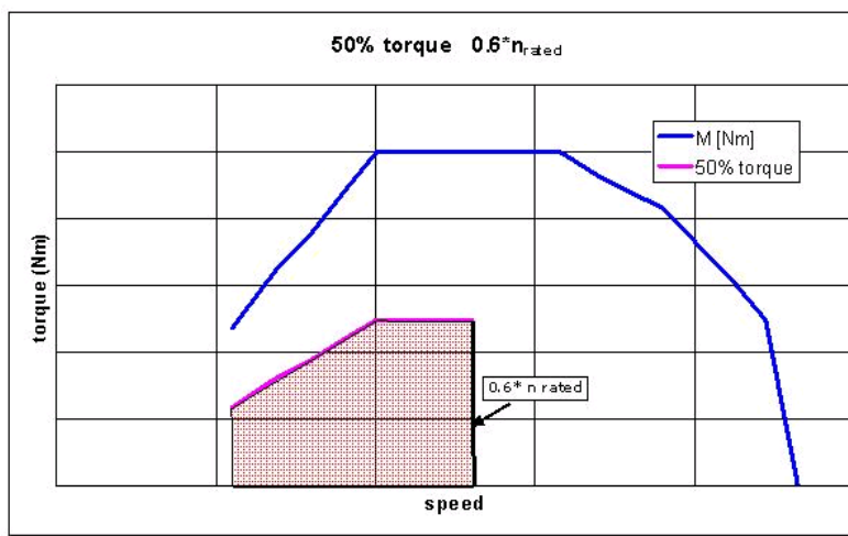
Figure A.9-2. Severe inducement torque reduction scheme
