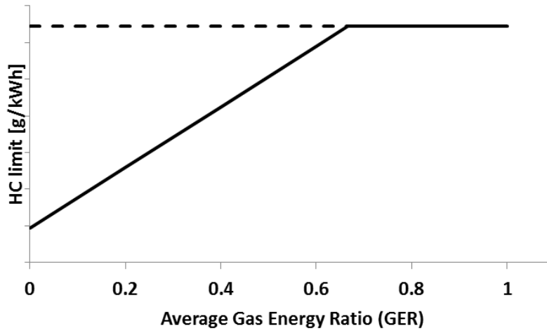
Diagram showing HC emission limit as function of average GER
