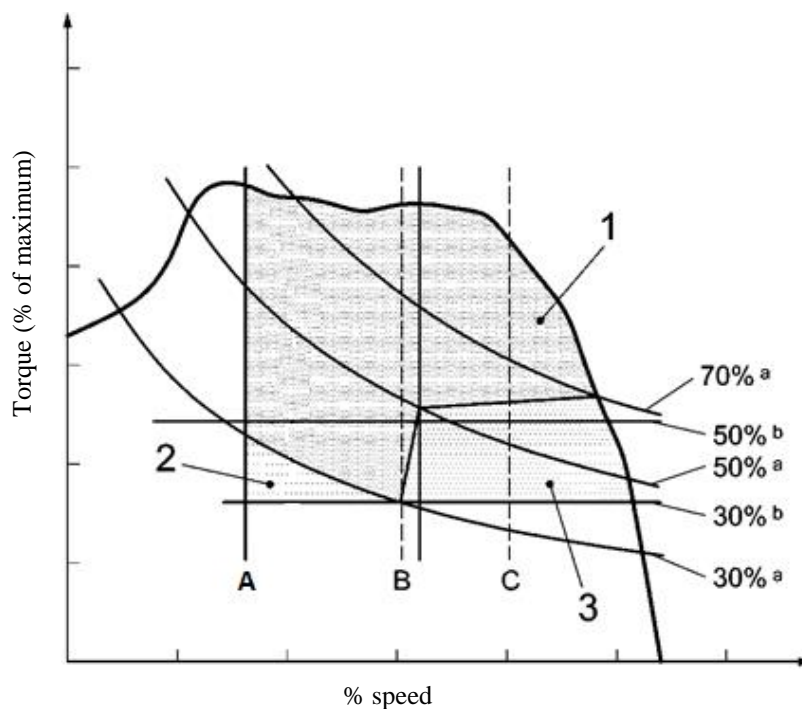
Figure 3. Control area for variable-speed engines of category NRE with maximum net power < 19 kW and speed C ≥ 2400 rpm
