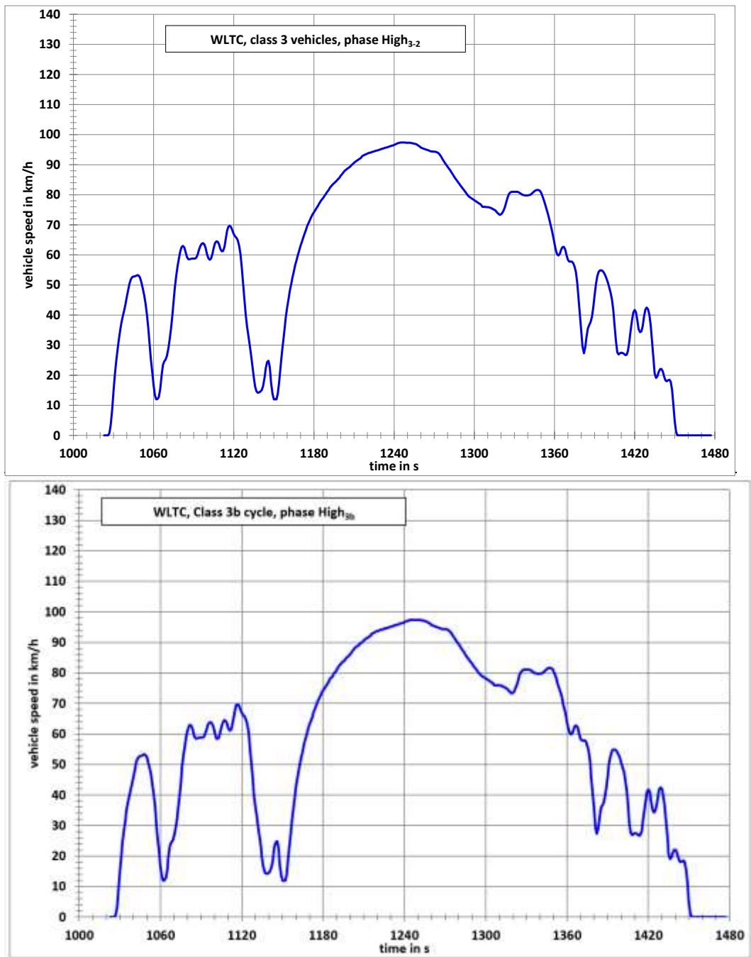
Figure A1/11 WLTC, Class 3b vehicles cycle, phase High 3b-2
