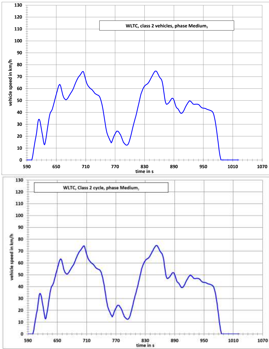
Figure A1/4 WLTC, Class 2 Vehicles cycle, Phase-phase Medium 2
