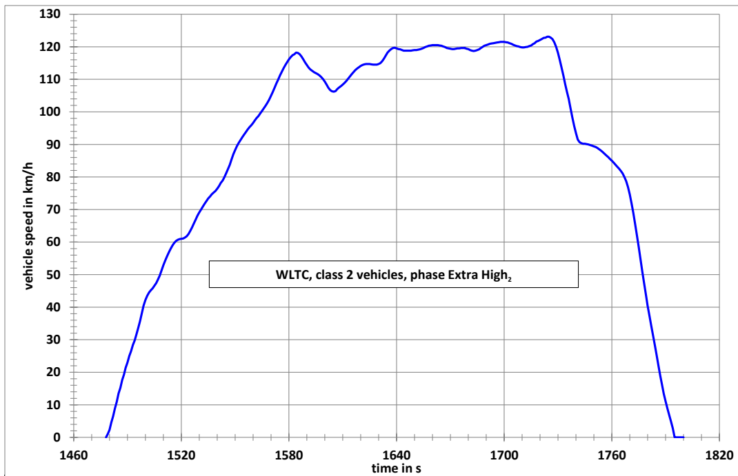
Figure A1/6 WLTC, Class 2 vehicles cycle, phase Extra High 2
