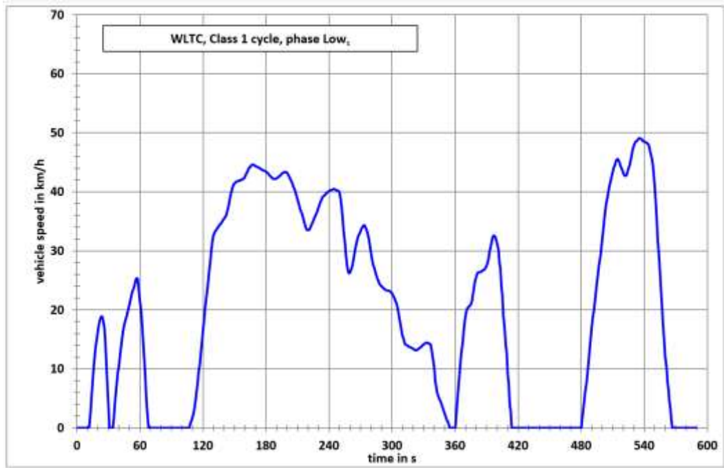
Figure A1/1 WLTC, Class 1 vehicles cycle, phase Low 1
