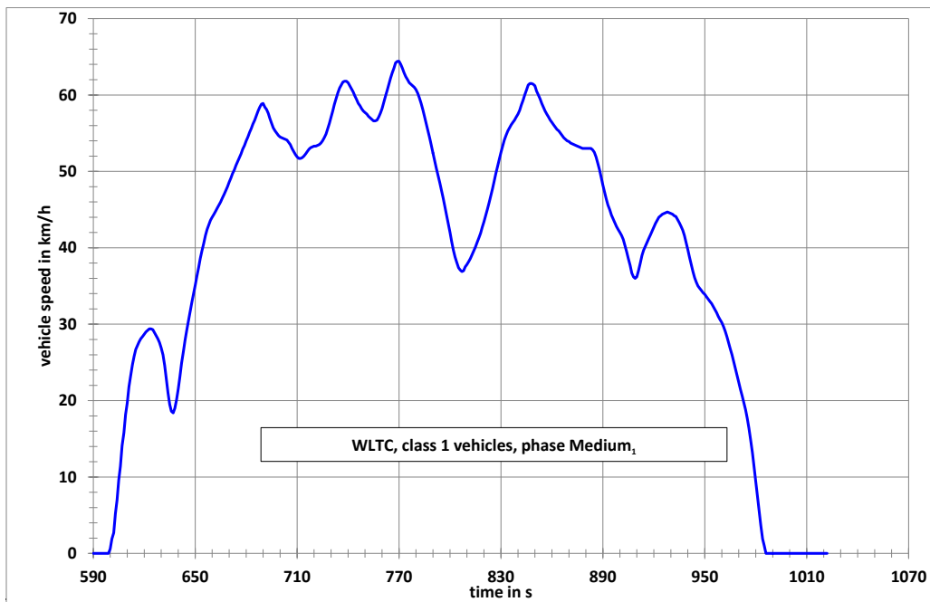
Figure A1/2 WLTC, Class 1 vehicles cycle, phase Medium 1
