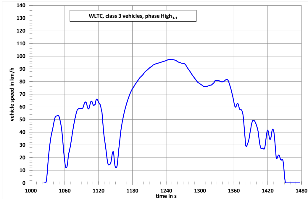
Figure A1/10 WLTC, Class 3a vehicles cycle, phase High 3a-1
