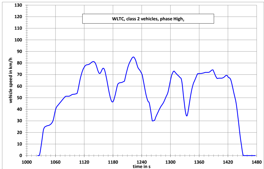
Figure A1/5 WLTC, Class 2 vehicles cycle, phase High 2
