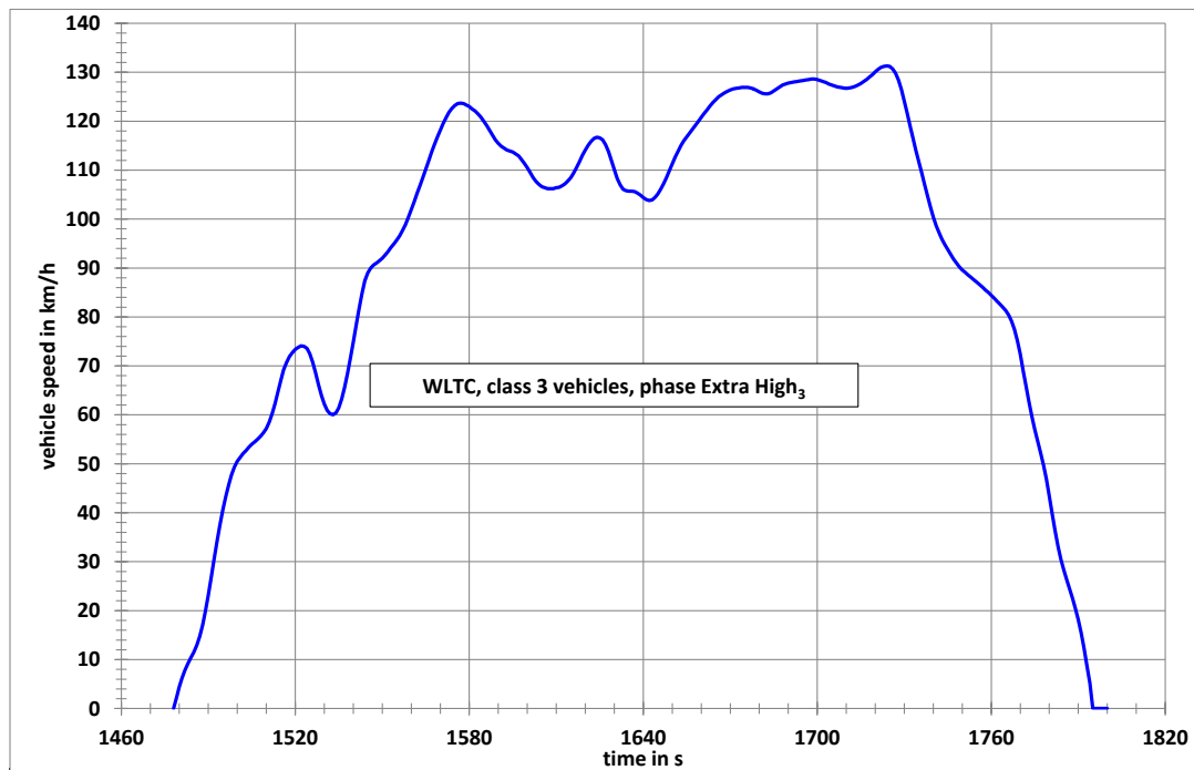
Figure A1/12 WLTC, Class 3 vehicles cycle, phase Extra High 3
