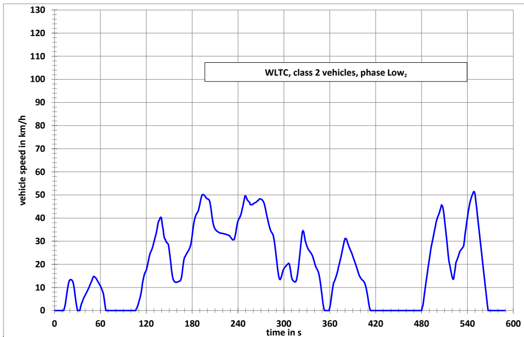
WLTC, Class 2 vehicles cycle, phase Low 2
