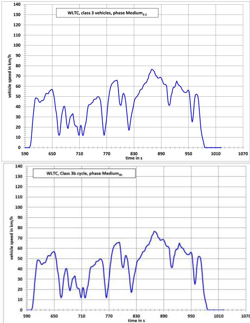
Figure A1/9 WLTC, Class 3b vehicles cycle, phase Medium 3b-2
