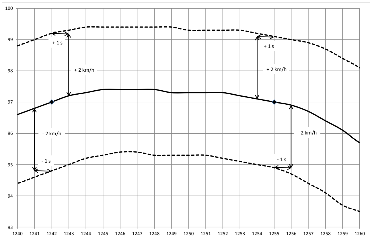
Figure A6/2 Speed trace tolerances
