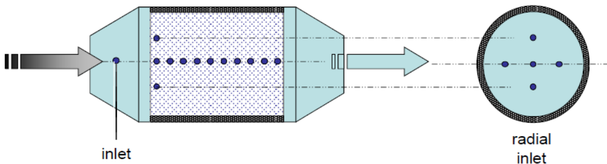
Figure 1 Example of temperature sensors location in a generic after-treatment device
