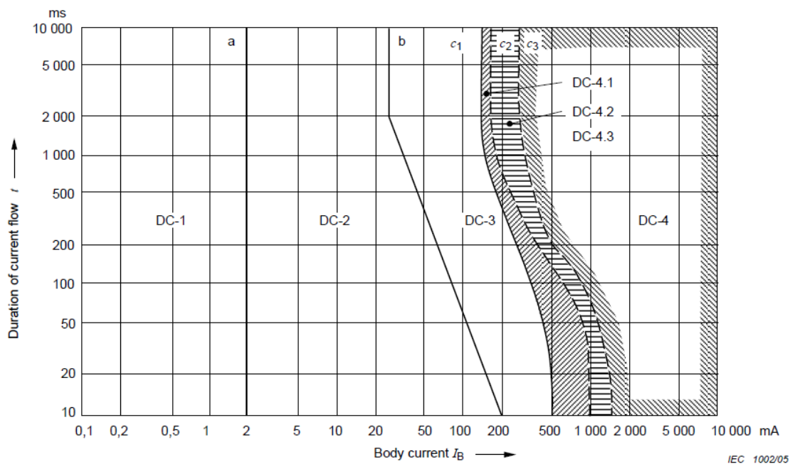
Figure 12 Conventional time/current zones of effects of DC currents on persons for current path corresponding to left hand to feet (Figure 22 from IEC TS 60479-1)
