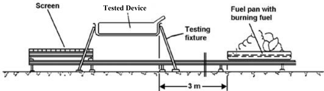
Figure 24 Phase A: Pre-heating
