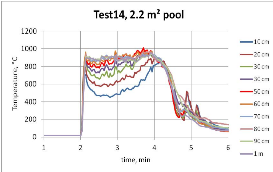
Figure 16. Temperature readings at different heights above a 2.2 m 2 pool fire
