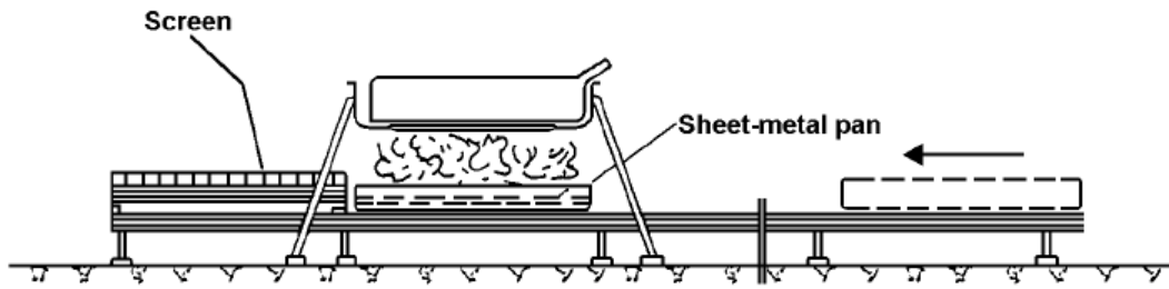
Figure 10 Phase B: Direct exposure to flame
