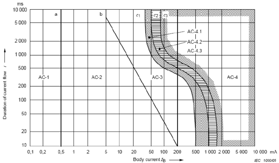
Figure 11 Conventional time/current zones of effects of AC currents (15Hz to 100 Hz) on persons for current path corresponding to left hand to feet (Figure 20 from IEC TS 60479-1)
