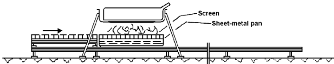
Figure 26 Phase C: Indirect exposure to flame
