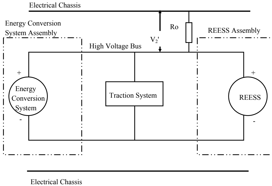
Figure 20 Measurement of V_2'
