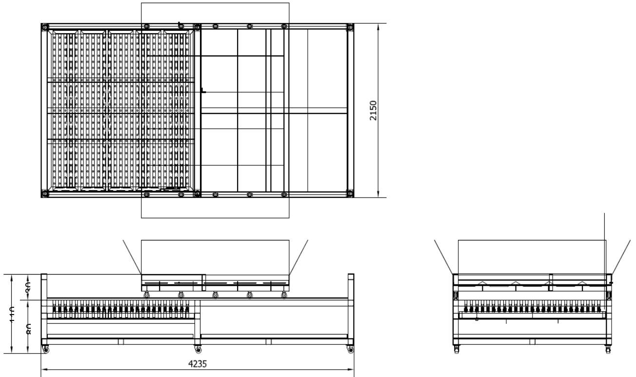
Figure 18 Illustration of KATRI LPG Burner
