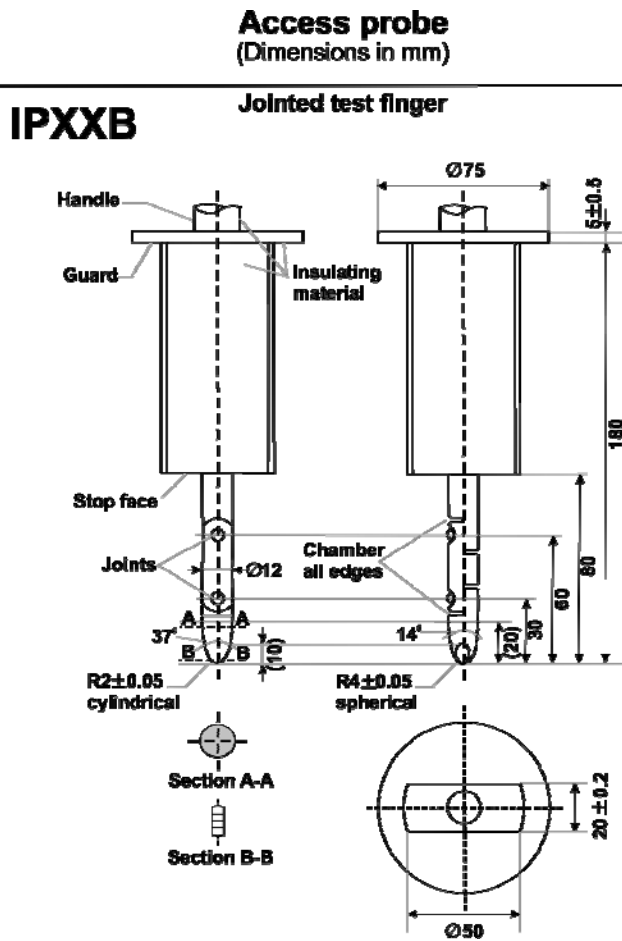
Figure 22 Jointed Test Finger
