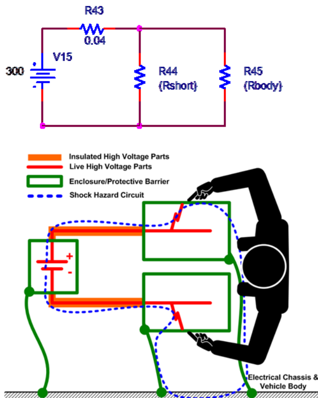
Figure 10 Potential risk scenario of indirect contact
