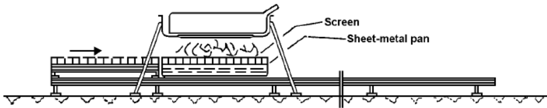
Figure 11 Phase C: Indirect exposure to flame
