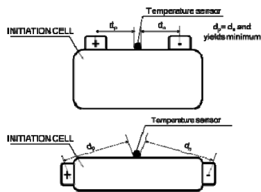
Figure 2 Example of set positions of temperature sensor in Overcharge
