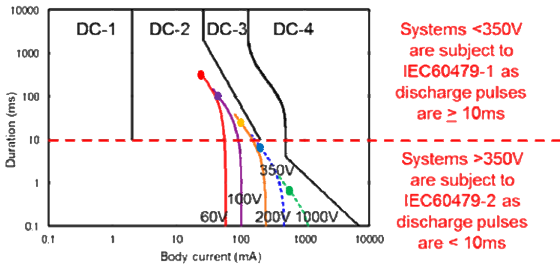
Figure 9 Root Mean Square Body Current (IRMS), 0.2J Capacitors, Large area/wet/hand-to-hand body resistance
