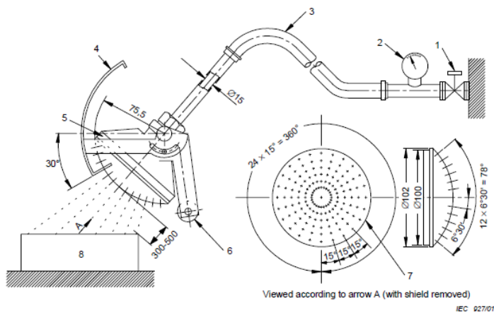
Figure 2 Splashing test nozzle
