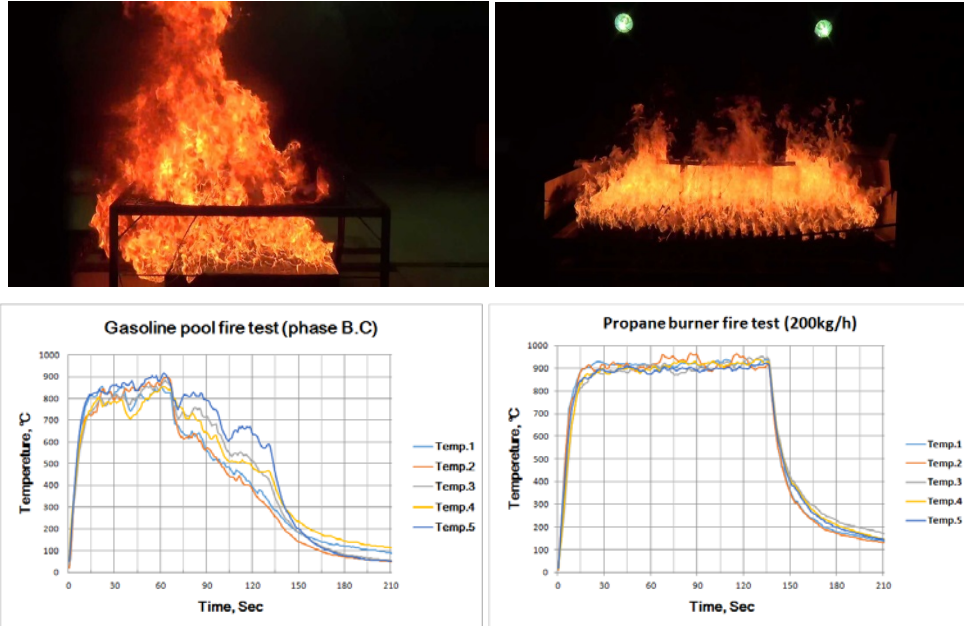
Test scene photographs and temperature measurements of a gasoline pool fire and an LPG burner fire
