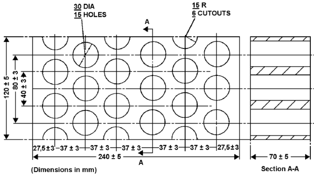
Figure 13 Dimension of Firebricks
