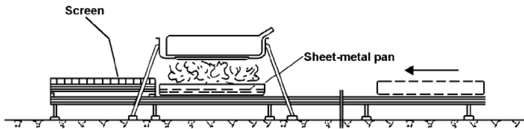
Figure 25 Phase B: Direct exposure to flame
