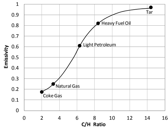
Figure 19 Emissivity of Different Fuel Flames 14
