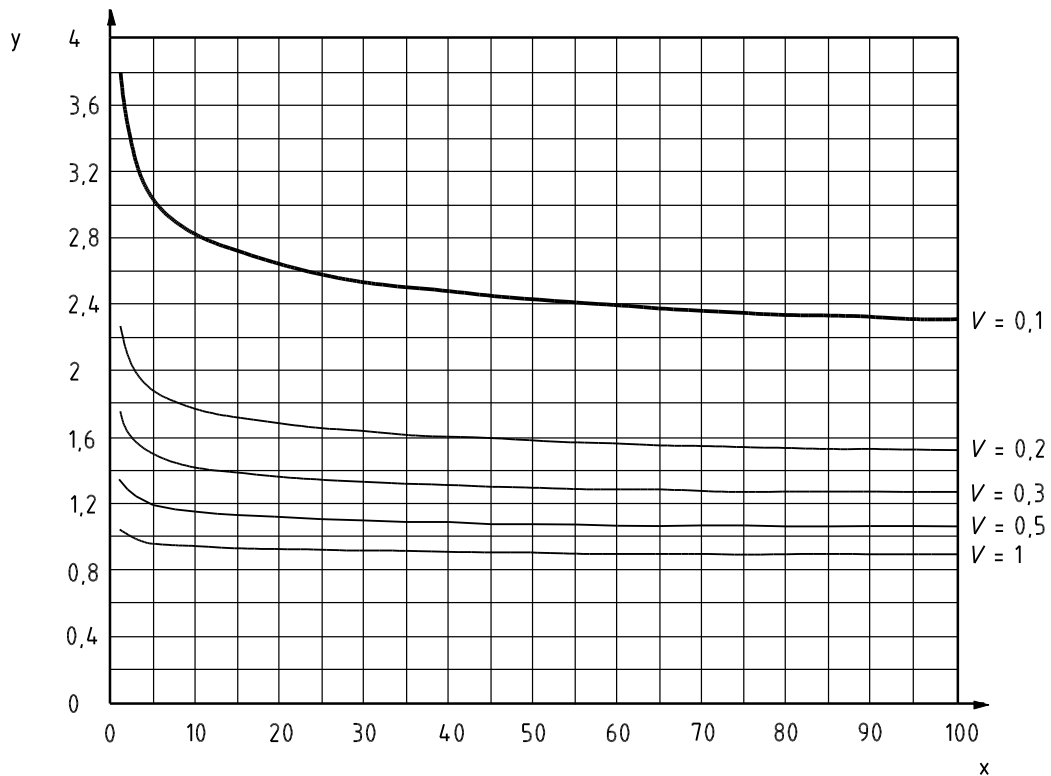
Figure D.2 – Minimum character height as function of adaptation luminance for selected visual acuities V ; viewing distance S_e = 100 \text{ mm}
