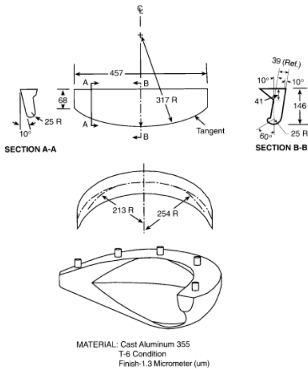
Figure 3 Bead unseating block
