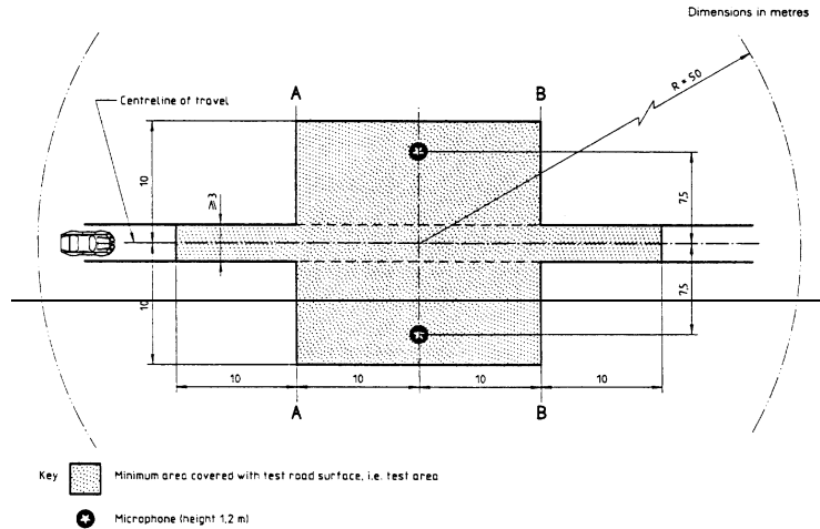
Figure 1 Minimum requirements for test surface area (The shaded part is called "Test Area")
