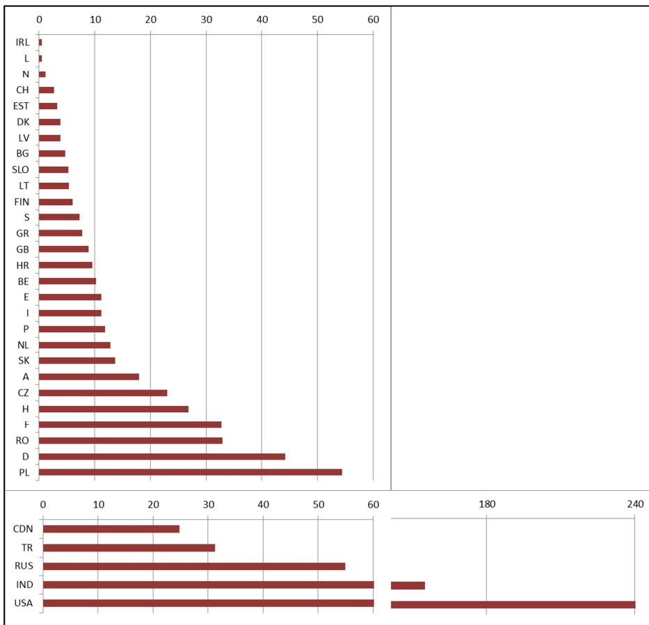
Figure 10 (pc11) Number of level crossing fatalities in significant accidents (pc2) , “ERA” and fatal accidents in “other” countries , annual average of 2006-2014
