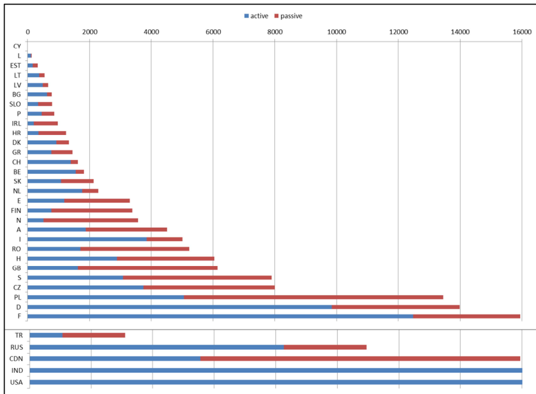
Figure 1 Number of level crossings, “ERA” and “other” countries, 2014
