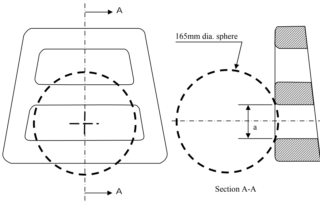
Figure 8-2 - Measurement of a horizontal gap "a".
