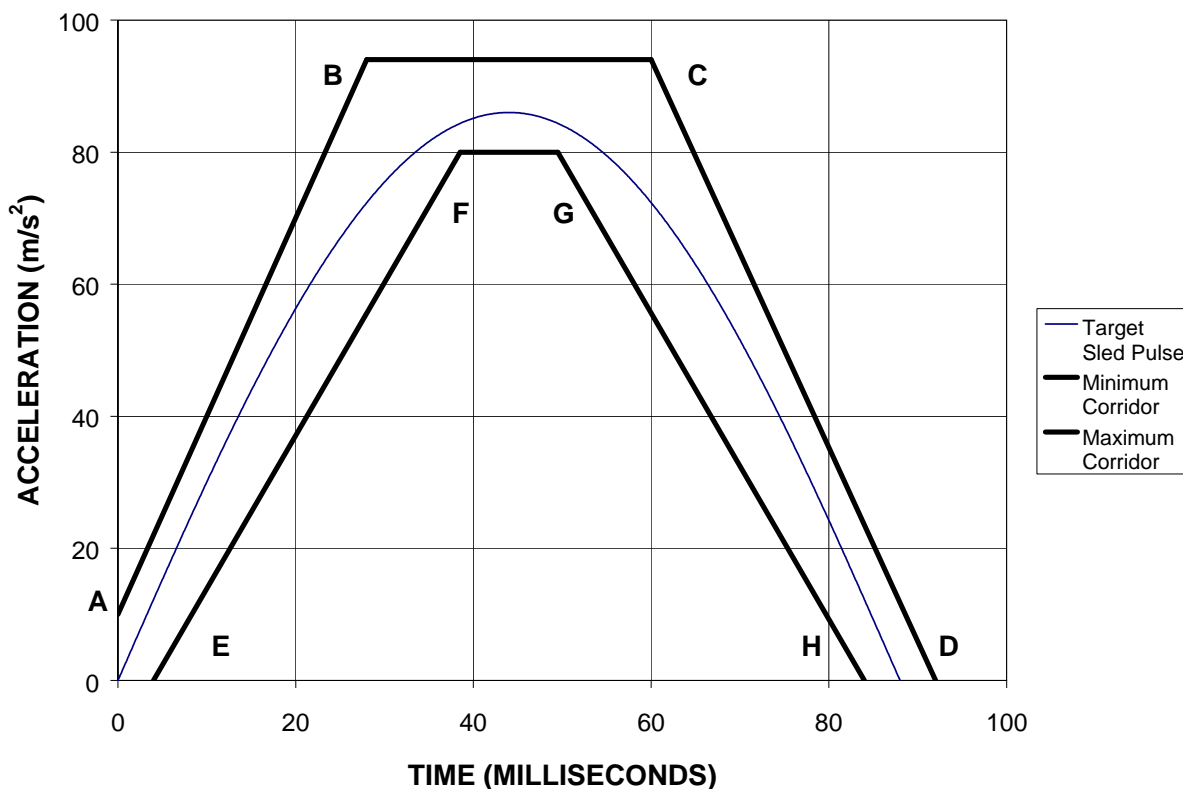
Figure 14-1 Sled pulse acceleration corridor.
