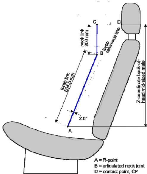
Figure 10-1 [Goniometry in the test procedure using apparatus that facilitate the measurement of coordinates.]
