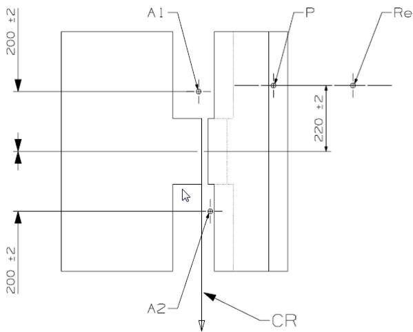
Figure 4 Side View – Bench with belt anchorages (Tolerance general: \pm 2 mm)
