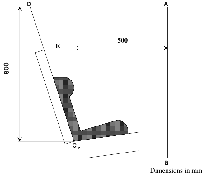
Arrangement for testing a forward-facing device
