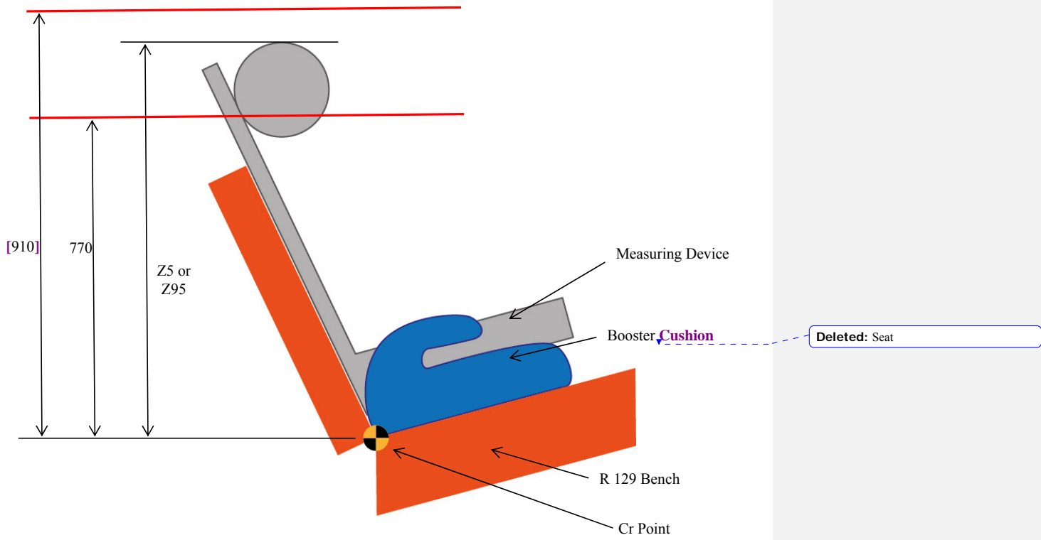
Figure 2 – Installation of the Measuring Device to measure Z5 and Z95
