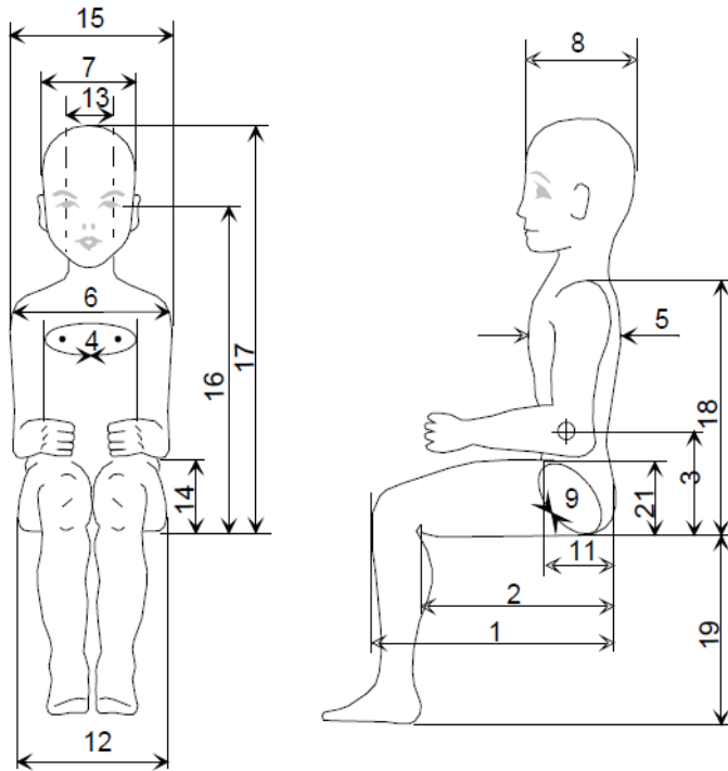
Main dimensions of dummy
