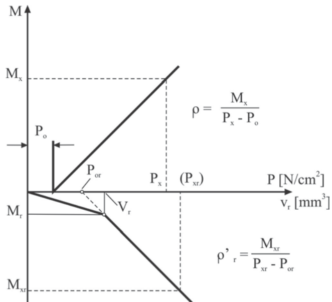
Figure 7 Hydraulic Brake (See paragraph 2. of this annex)
