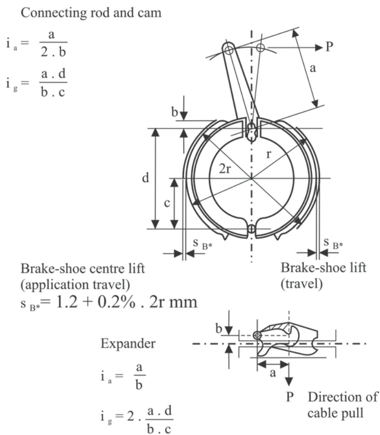
Figure 4 Brake checks (See paragraphs 2.2.22. and 2.3.4. of this annex)
