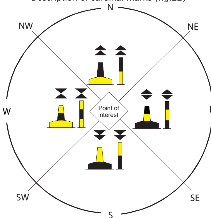
Description of cardinal marks (fig.22)
