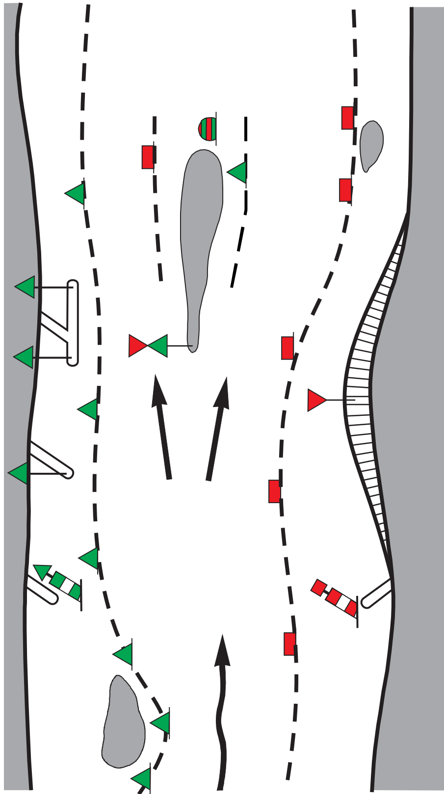
Example of use of the buoyage and marking described in chapters II and IV
